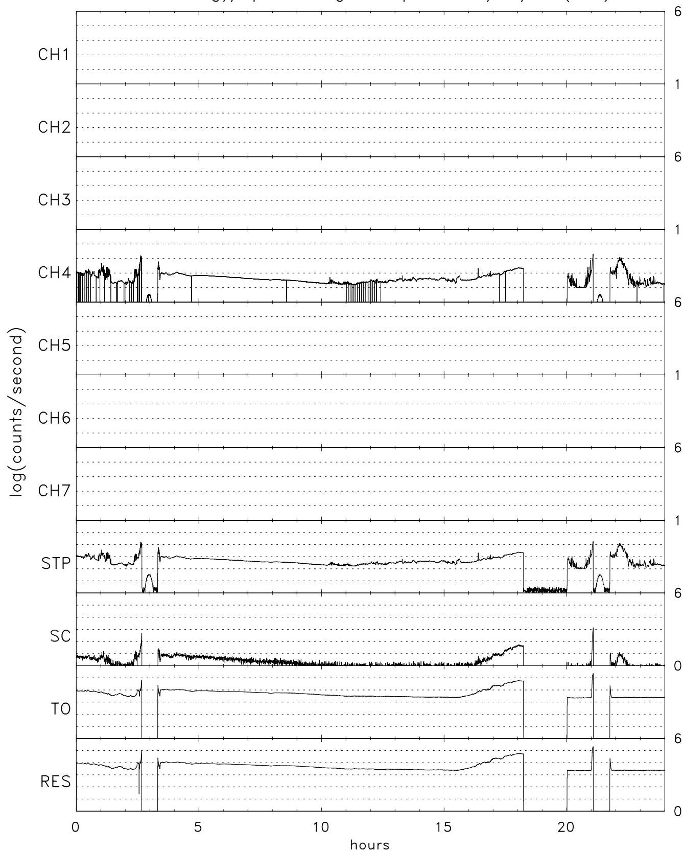
TIDE energy/spin averaged Stops for 10/27/03 (300)
