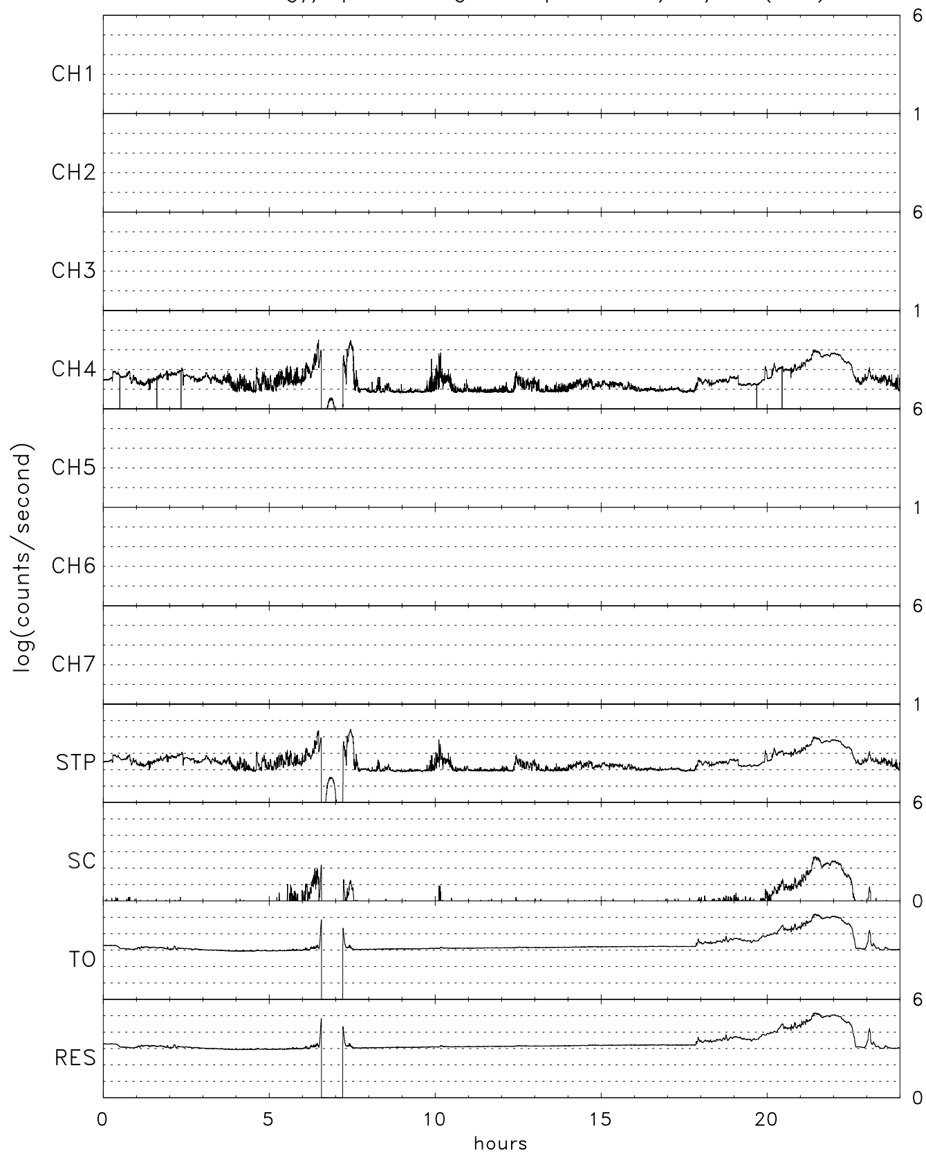
TIDE energy/spin averaged Stops for 09/17/03 (260)
