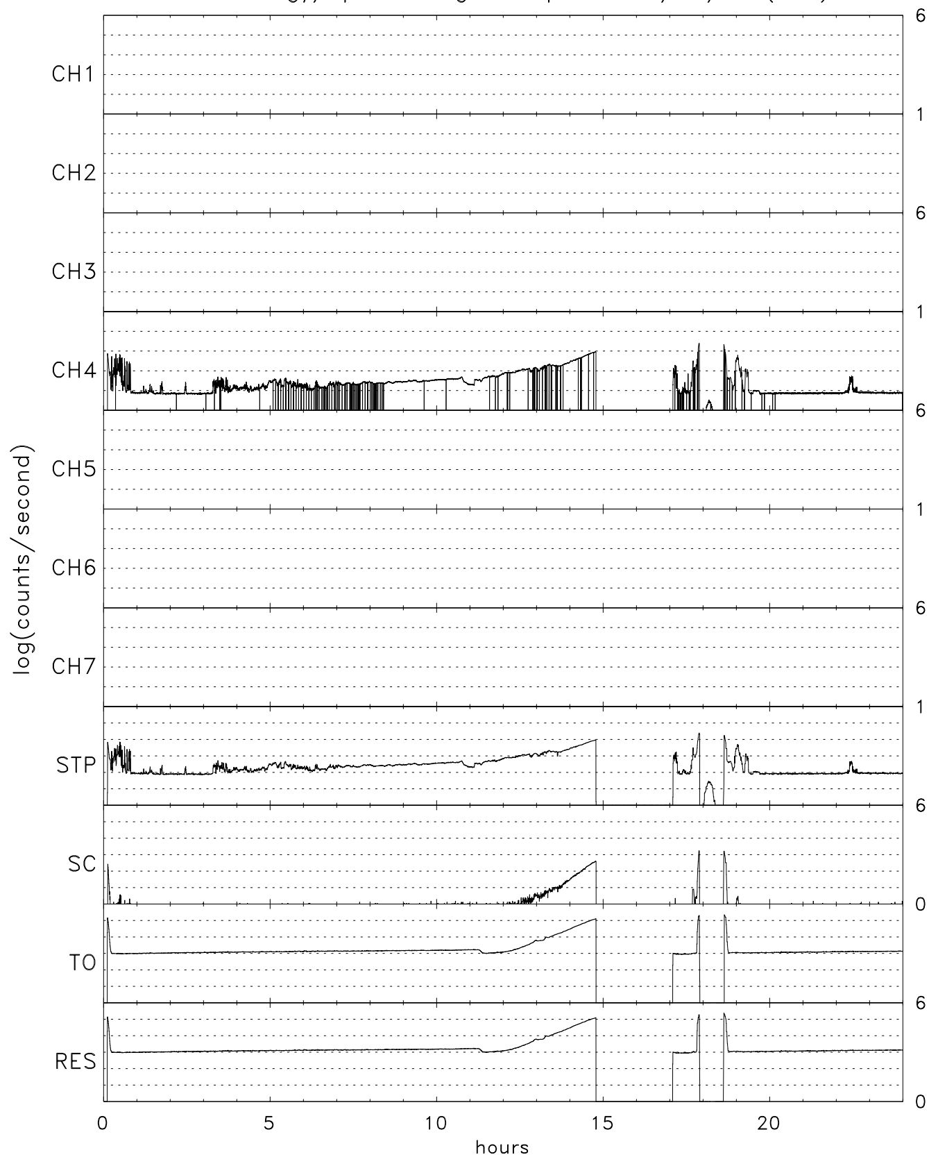
TIDE energy/spin averaged Stops for 09/15/03 (258)
