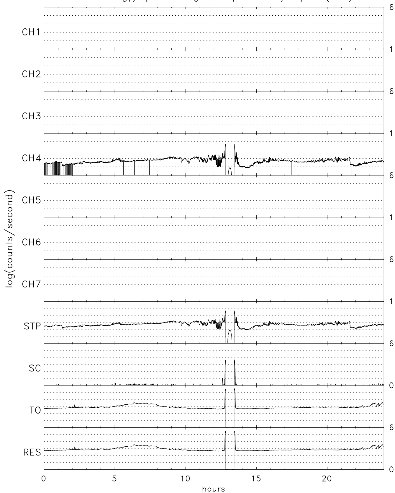
TIDE energy/spin averaged Stops for 06/13/03 (164)
