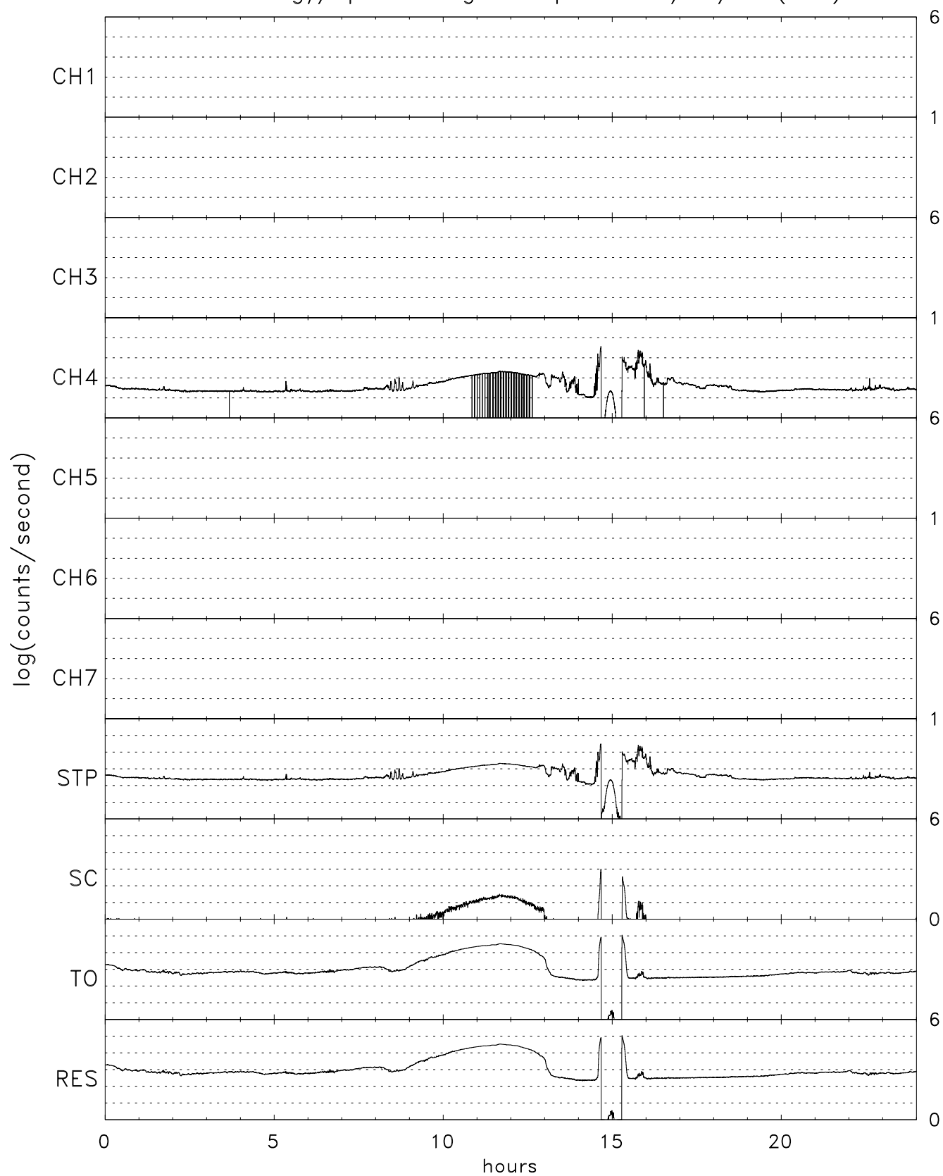
TIDE energy/spin averaged Stops for 12/16/02 (350)
