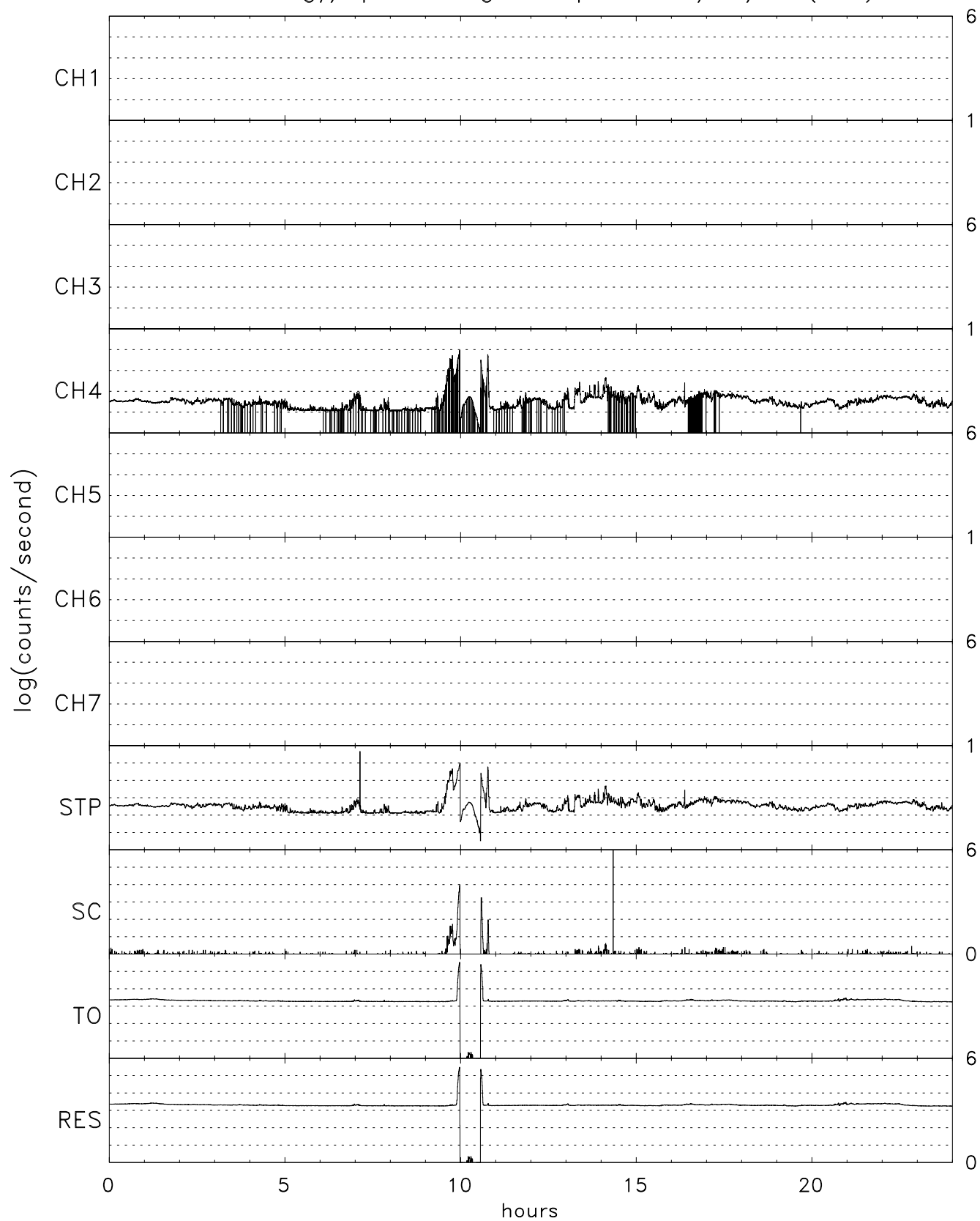
TIDE energy/spin averaged Stops for 08/26/02 (238)
