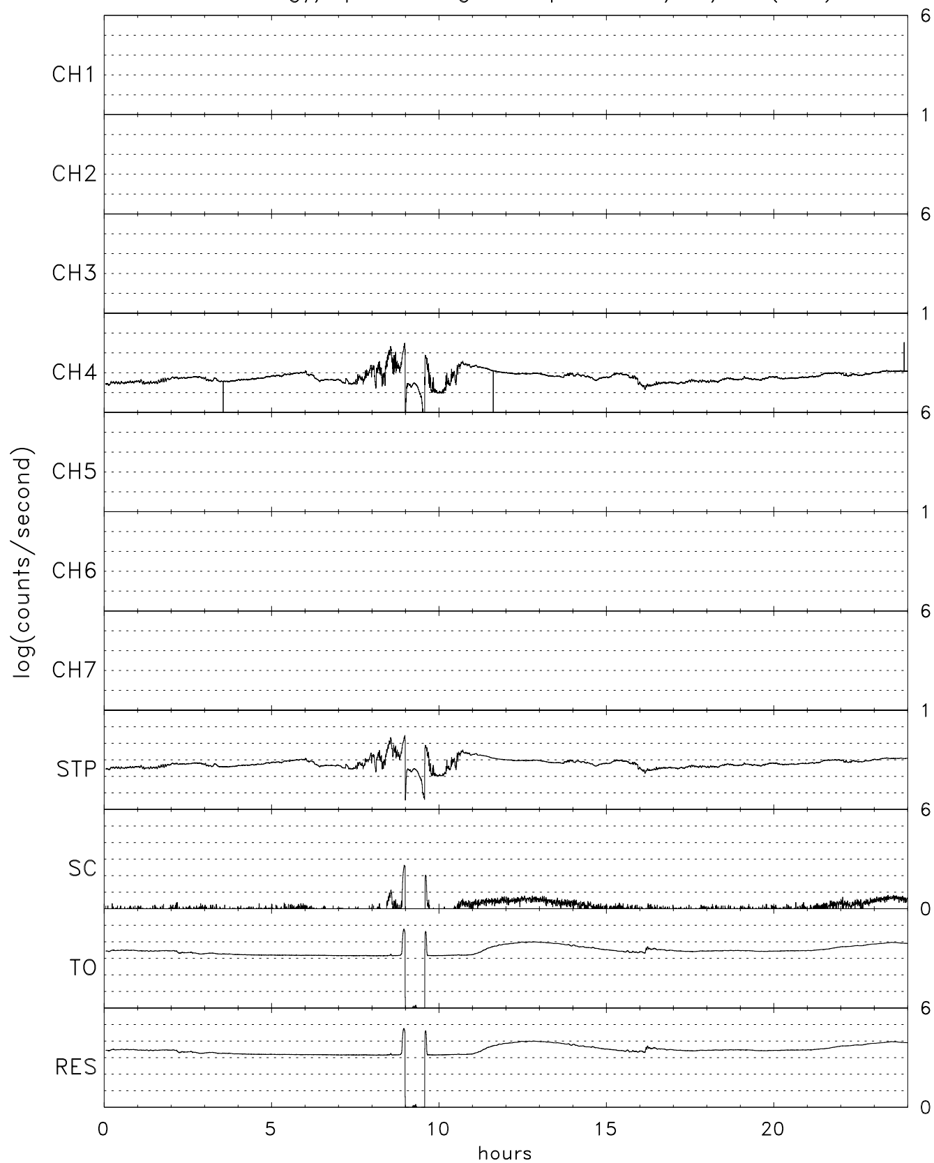
TIDE energy/spin averaged Stops for 06/26/02 (177)
