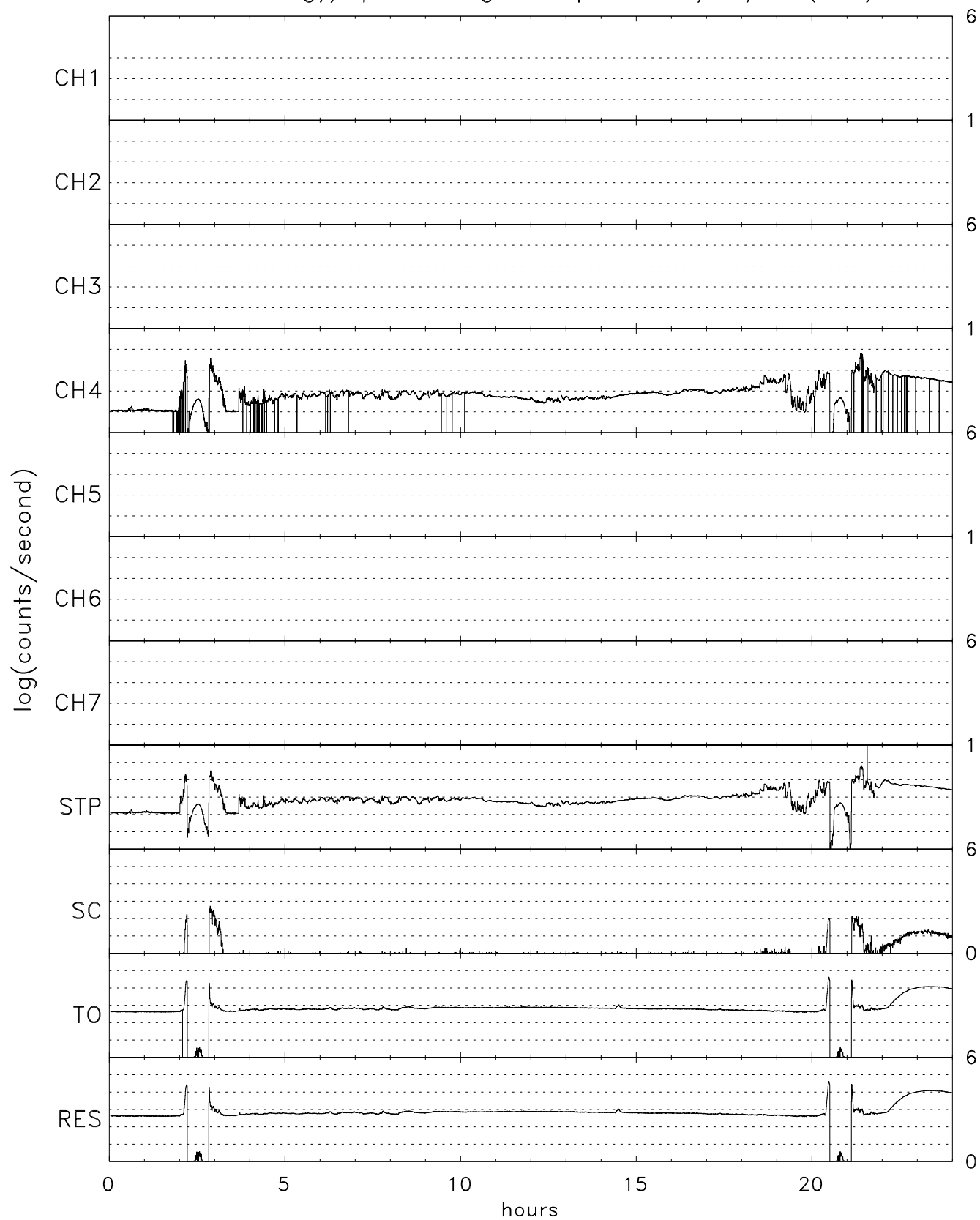
TIDE energy/spin averaged Stops for 12/13/01 (347)
