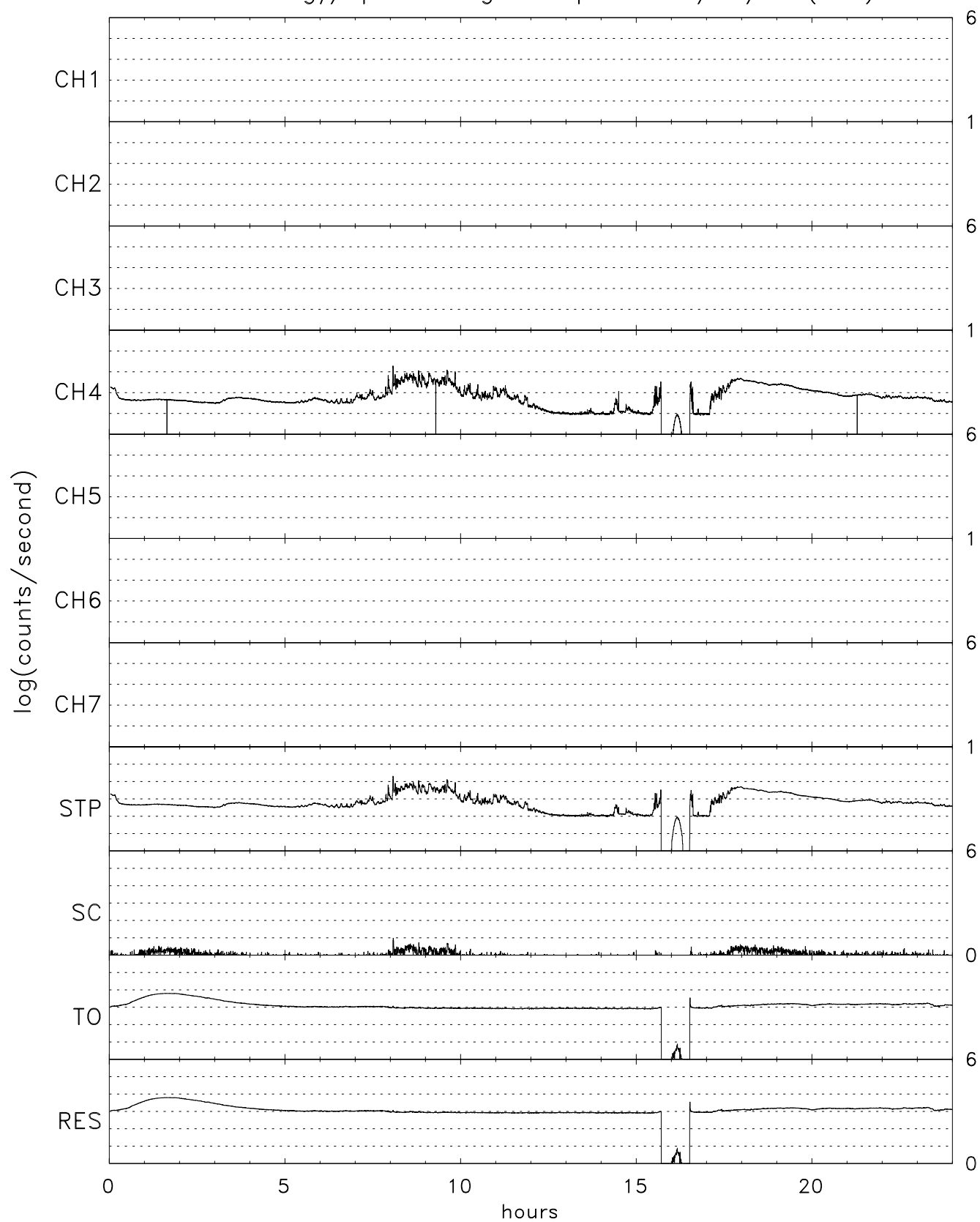
TIDE energy/spin averaged Stops for 06/17/01 (168)
