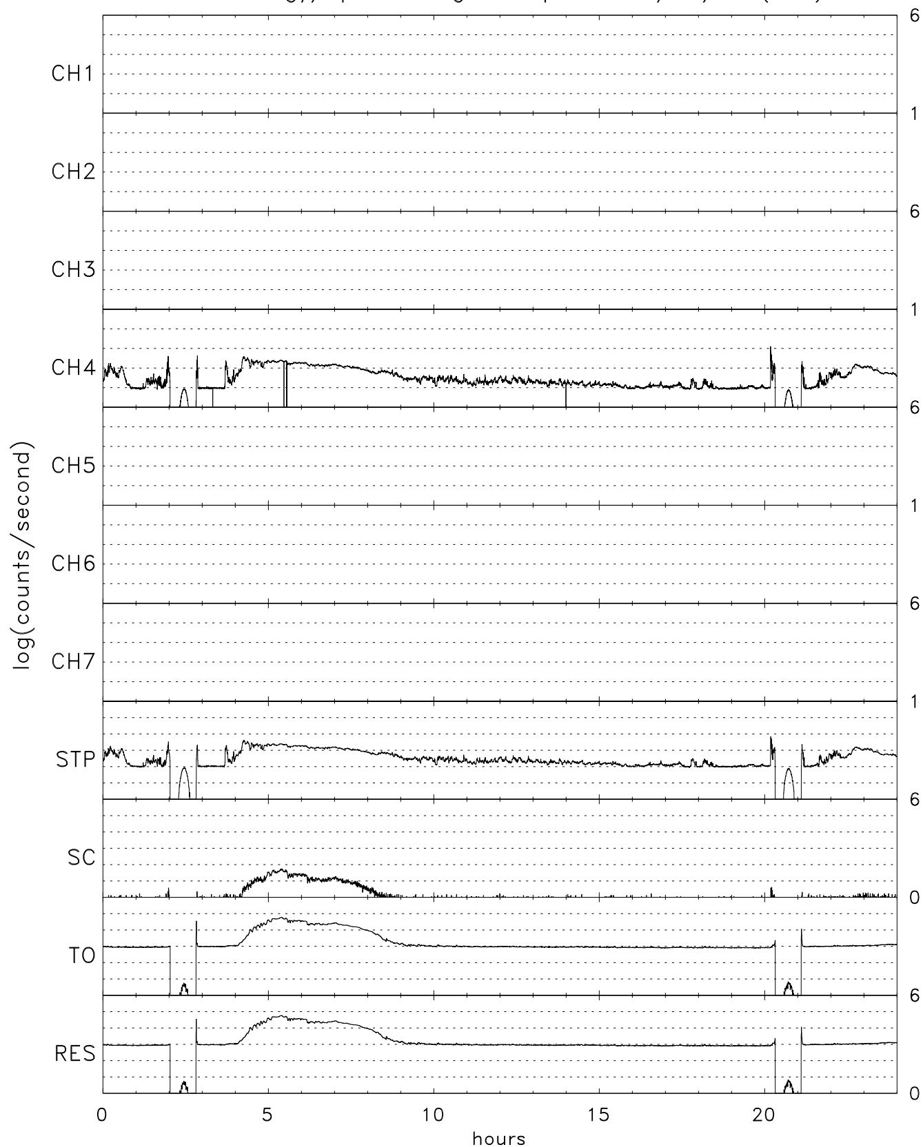
TIDE energy/spin averaged Stops for 06/13/01 (164)
