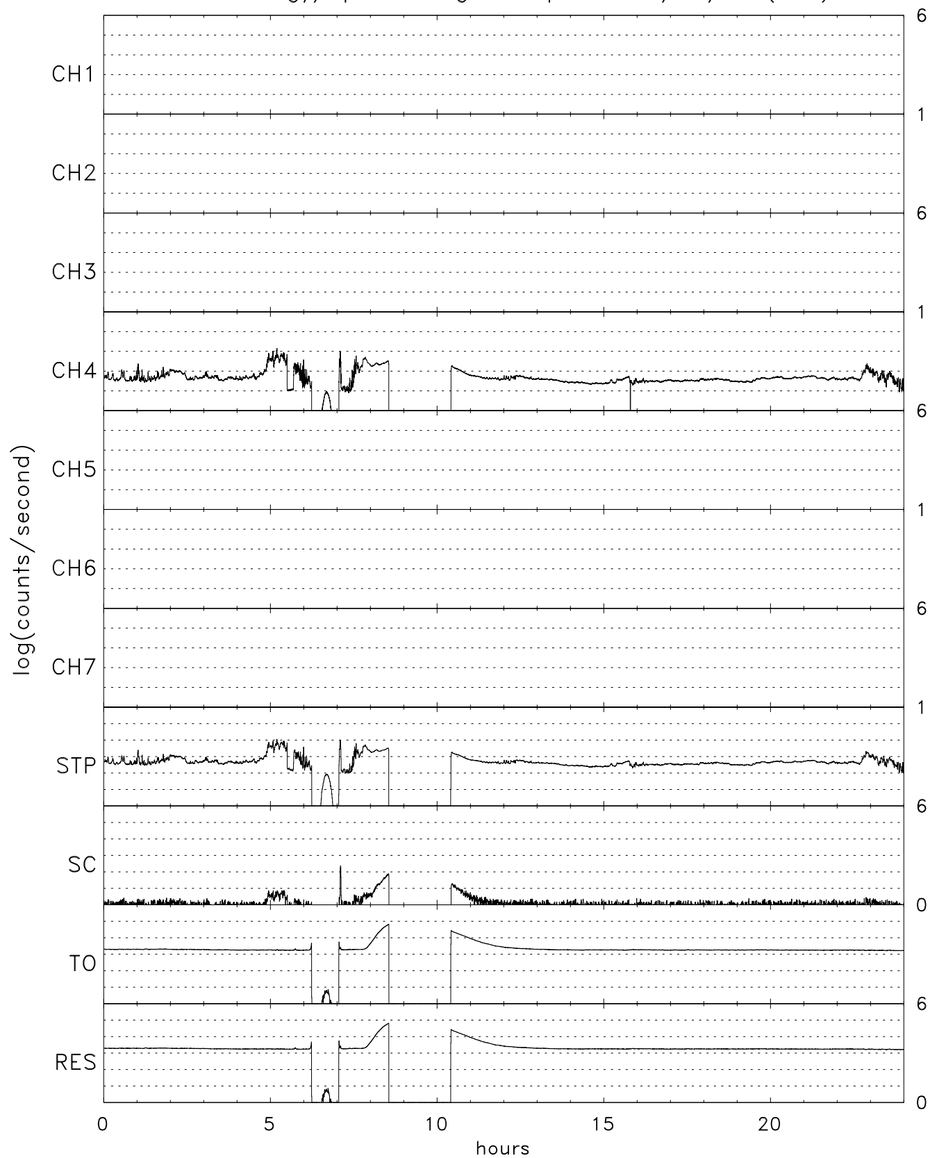
TIDE energy/spin averaged Stops for 05/24/01 (144)
