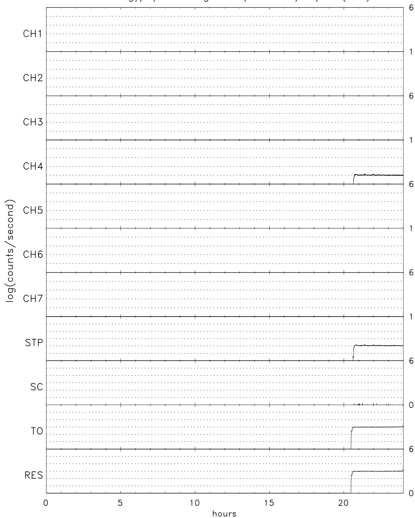
TIDE energy/spin averaged Stops for 12/20/00 (355)
