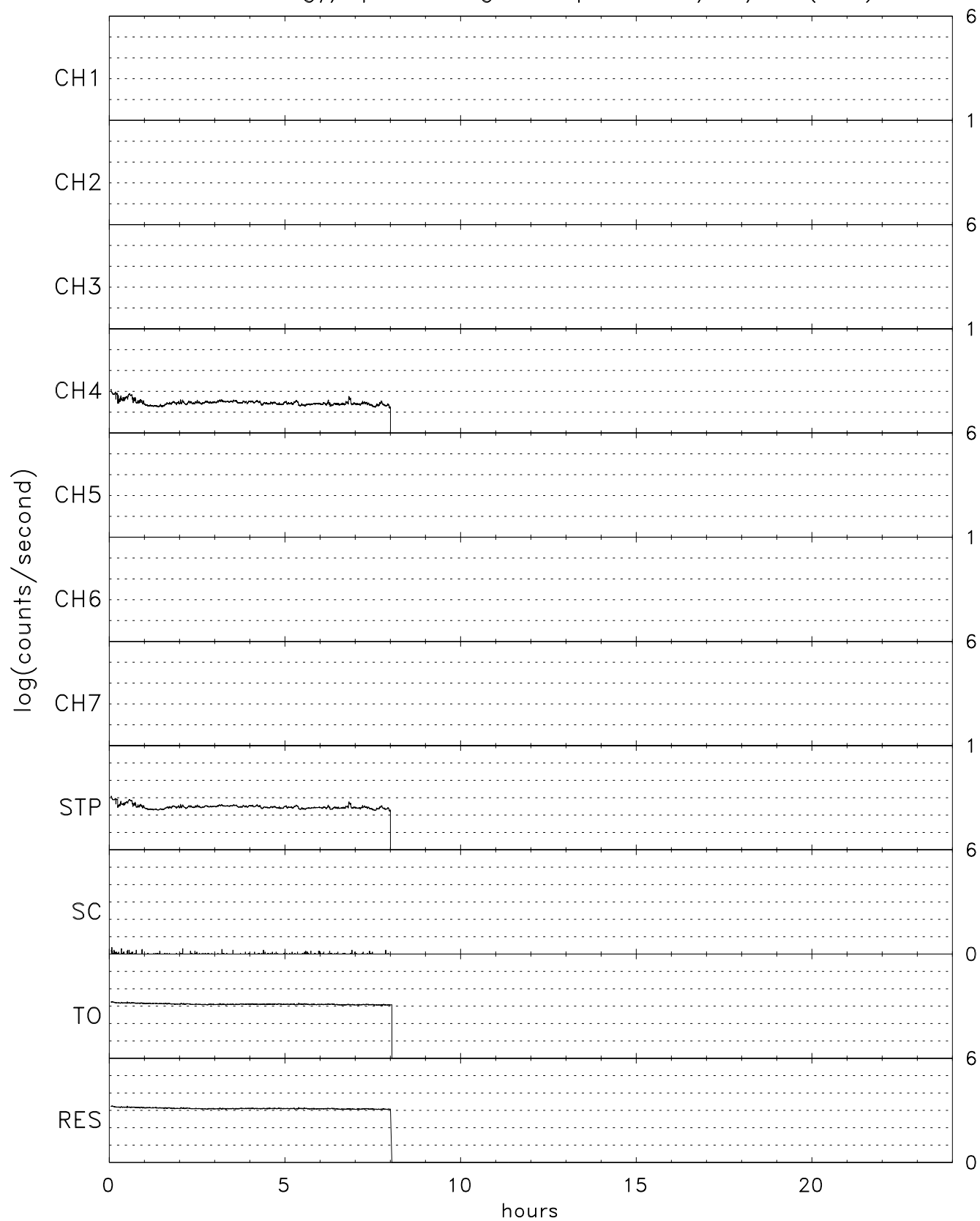
TIDE energy/spin averaged Stops for 12/19/00 (354)
