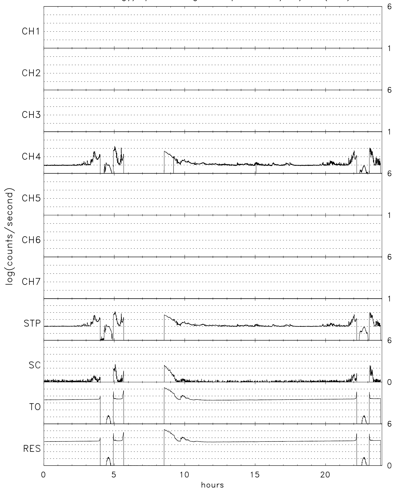
TIDE energy/spin averaged Stops for 09/27/00 (271)
