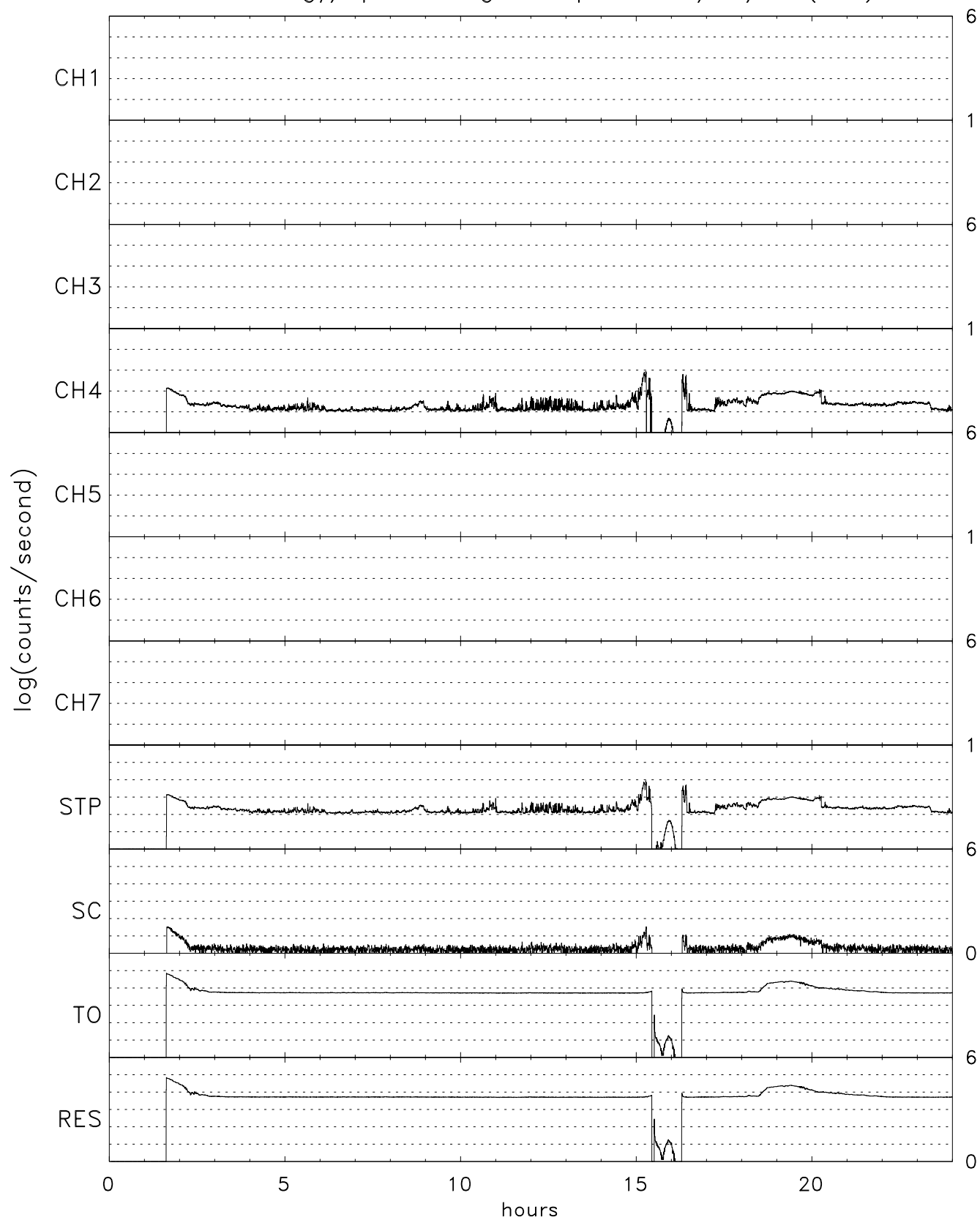
TIDE energy/spin averaged Stops for 09/19/00 (263)
