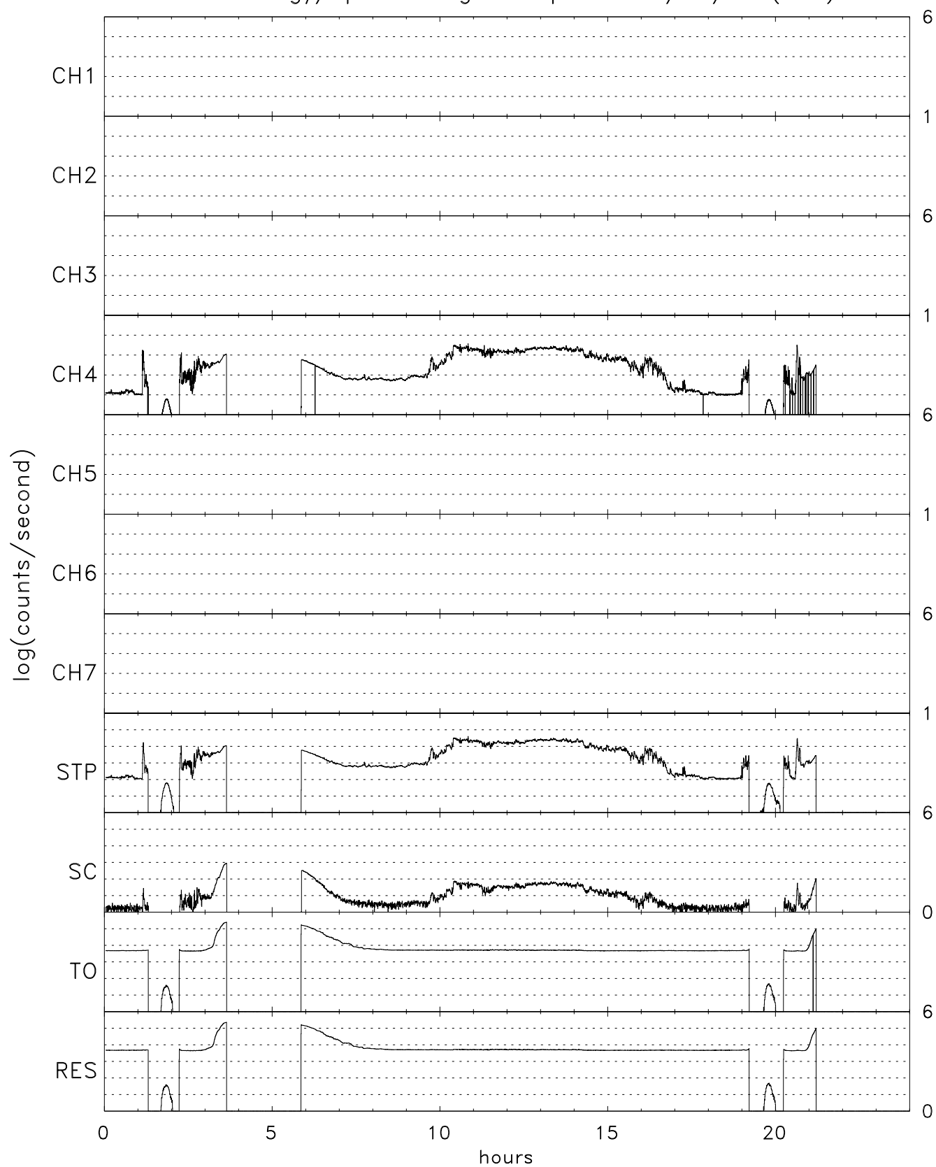
TIDE energy/spin averaged Stops for 05/07/00 (128)
