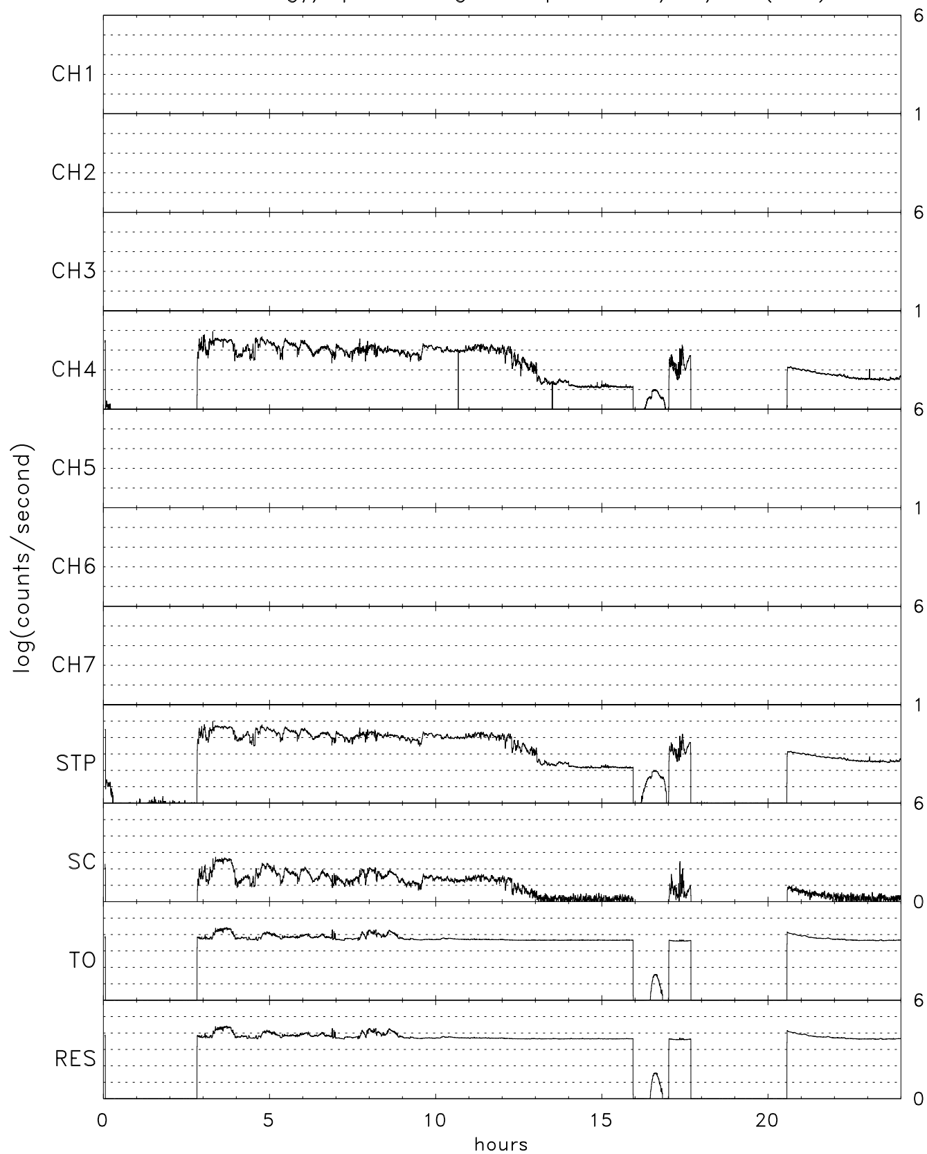
TIDE energy/spin averaged Stops for 04/07/00 (098)
