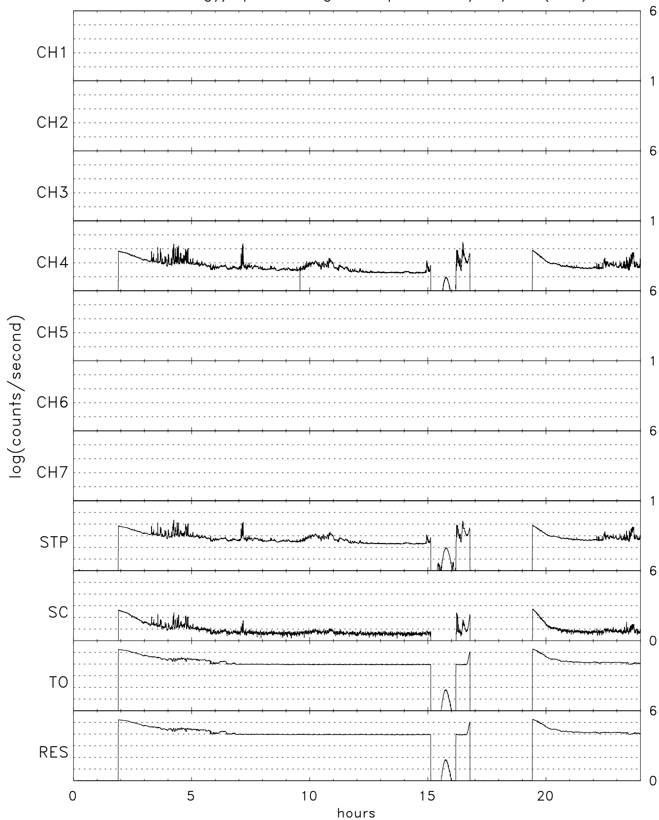
TIDE energy/spin averaged Stops for 02/25/00 (056)
