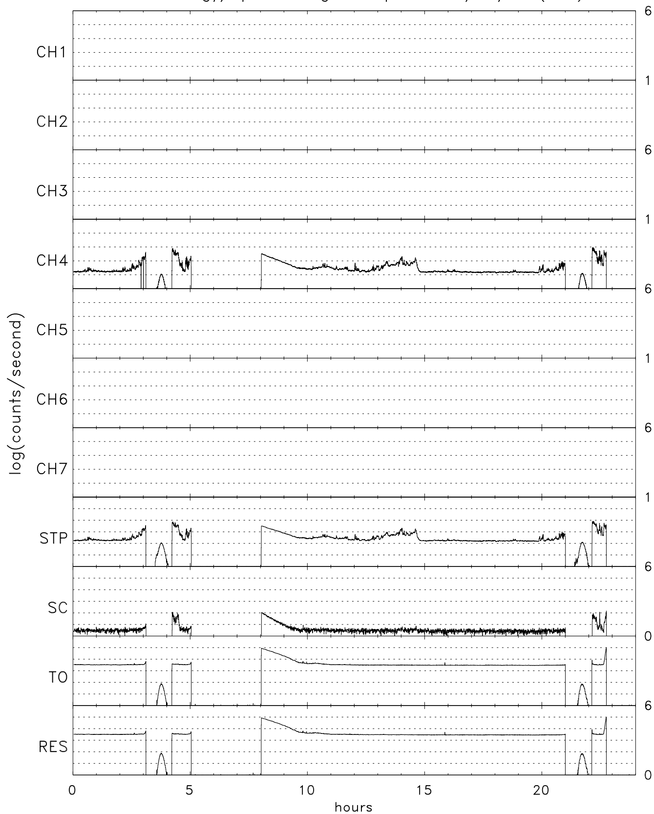
TIDE energy/spin averaged Stops for 01/07/00 (007)
