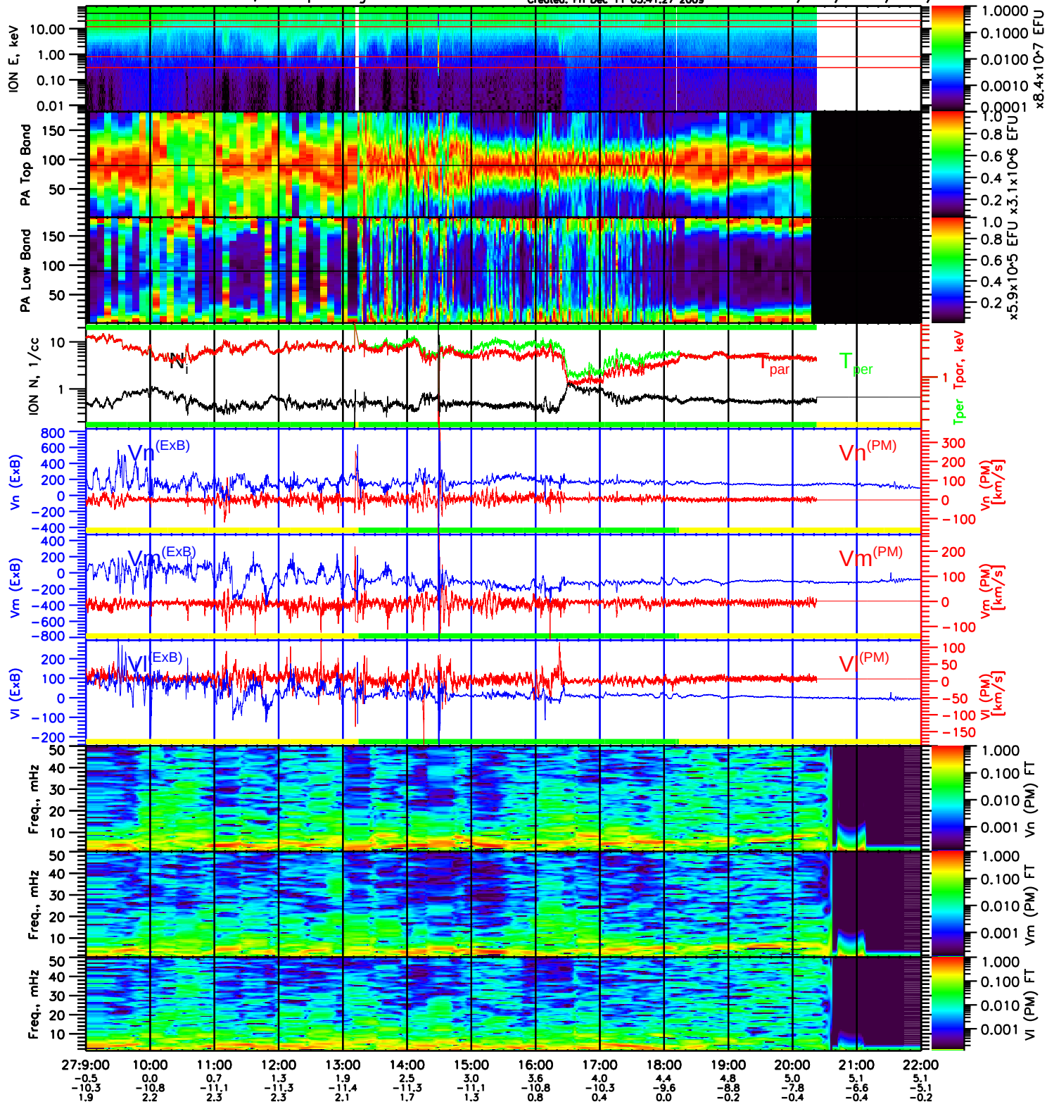
THEMIS-D 2007-10-27, Ion Spectrograms &amp; Moments.
