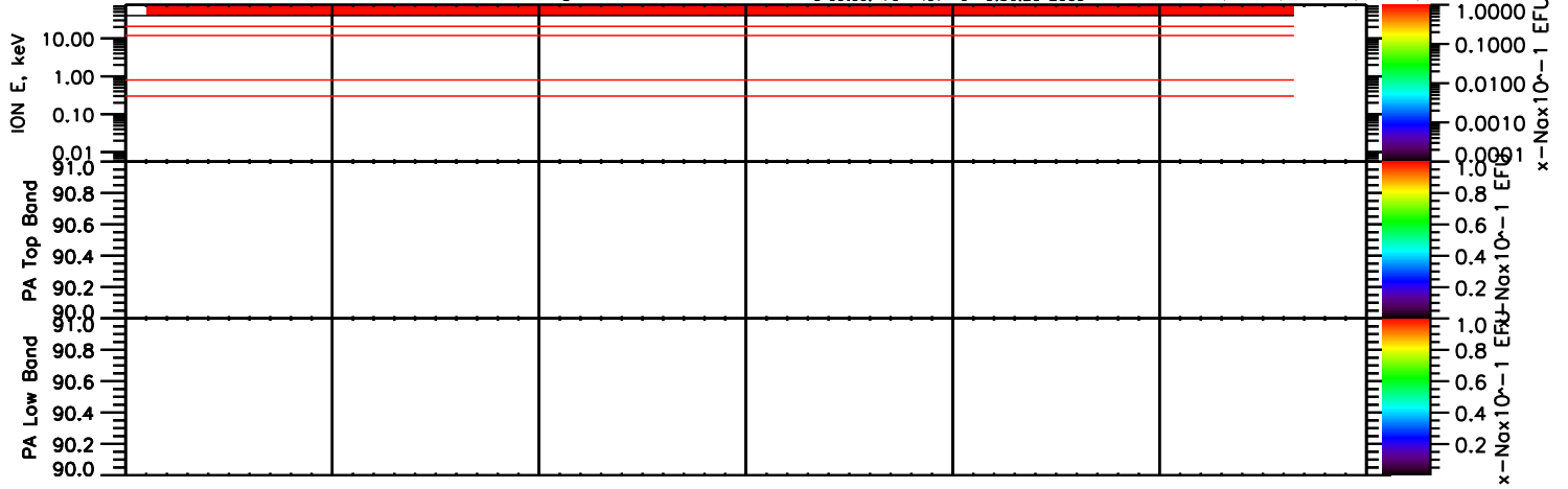
THEMIS-C 2007-10-6-13:00, Ion Spectrograms &amp; Moments.
