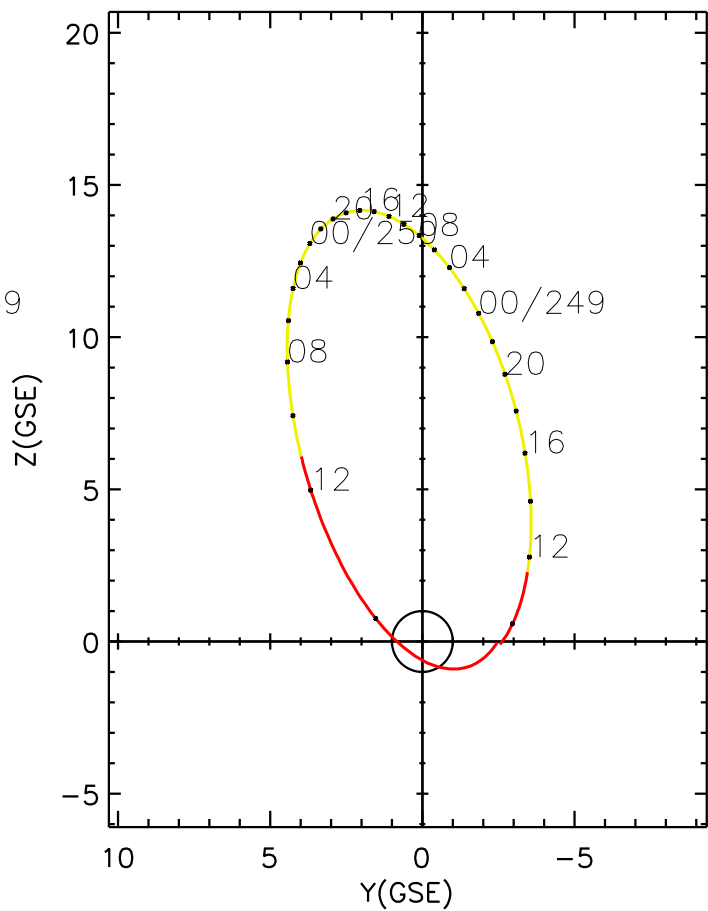
CLUSTER 2 orbit 2024 248 (09/04) 09:26 UT to 2024 250 (09/06) 15:31 UT
