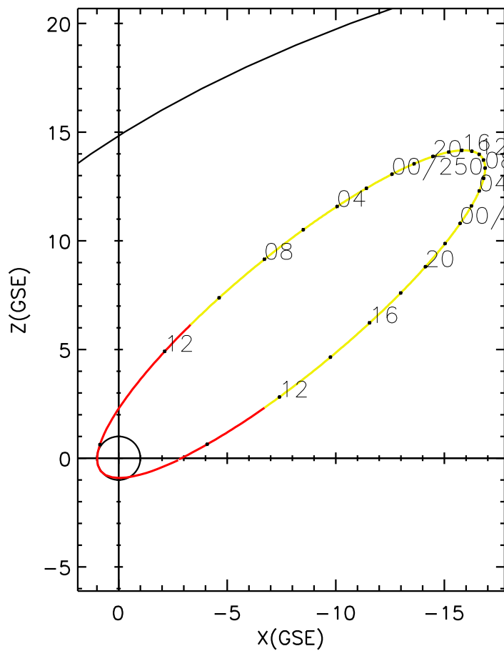
CLUSTER 2 orbit 2024 248 (09/04) 09:26 UT to 2024 250 (09/06) 15:26 UT
