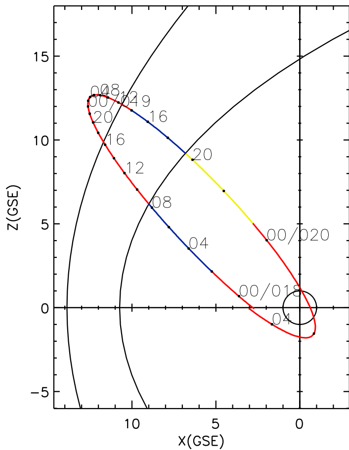
CLUSTER 2 orbit 2024 017 (01/17) 23:01 UT to 2024 020 (01/20) 05:16 UT
