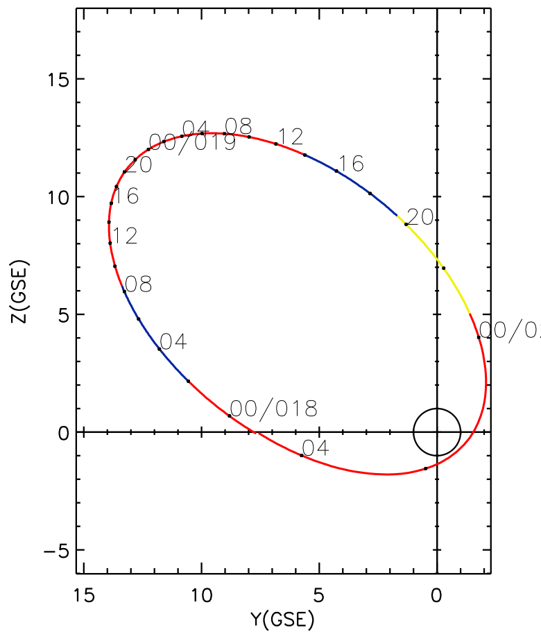
CLUSTER 2 orbit 2024 017 (01/17) 23:01 UT to 2024 020 (01/20) 05:16 UT
