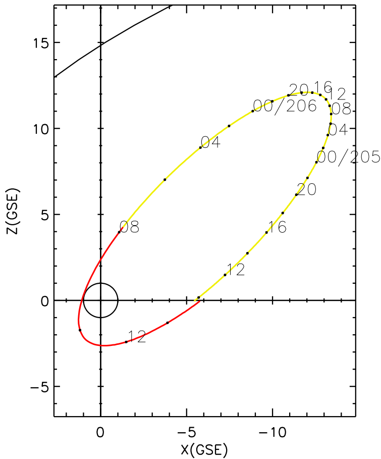
CLUSTER 2 orbit 2023 204 (07/23) 09:41 UT to 2023 206 (07/25) 15:56 UT
