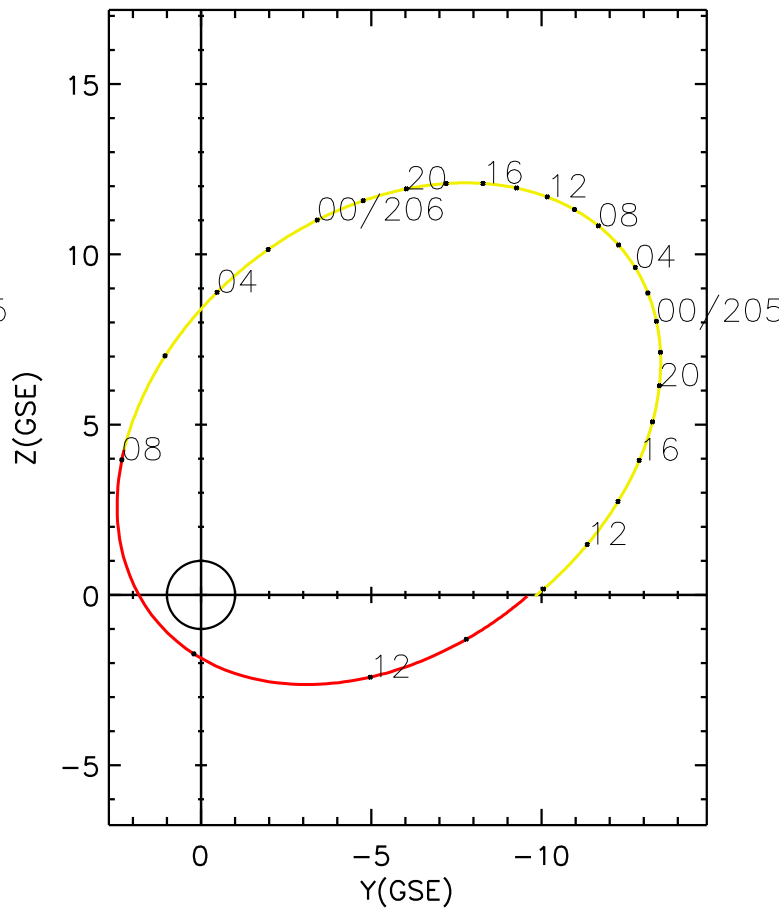
CLUSTER 2 orbit 2023 204 (07/23) 09:41 UT to 2023 206 (07/25) 15:56 UT
