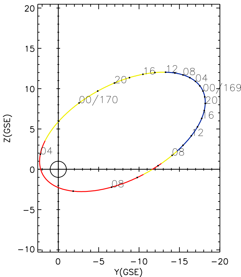
CLUSTER 2 orbit 2023 168 (06/17) 05:16 UT to 2023 170 (06/19) 11:31 UT
