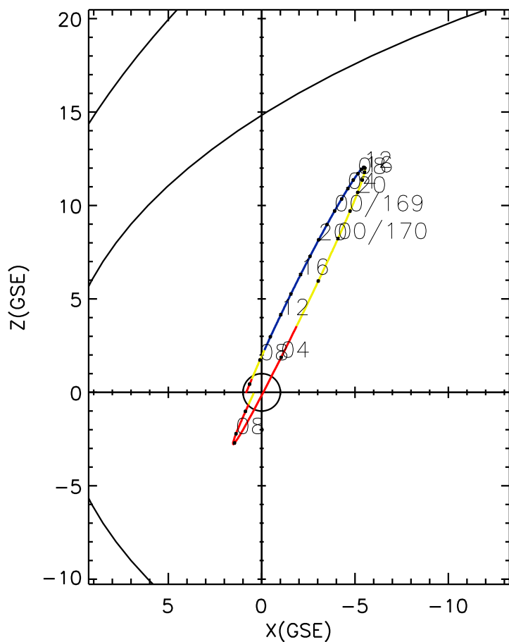
CLUSTER 2 orbit 2023 168 (06/17) 05:16 UT to 2023 170 (06/19) 11:31 UT
