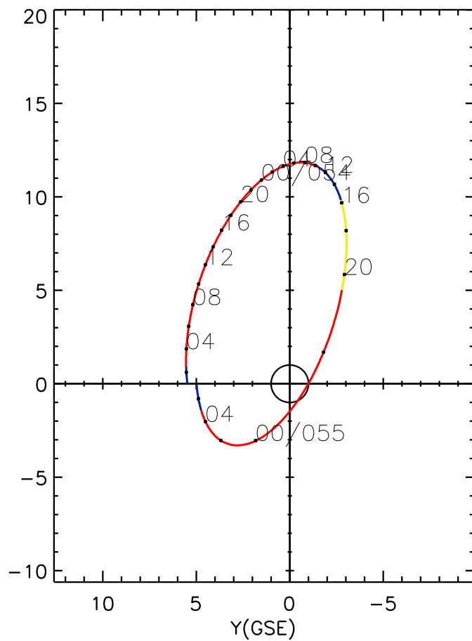
CLUSTER 2 orbit 2023 053 (02/22) 01:01 UT to 2023 055 (02/24) 07:11 UT
