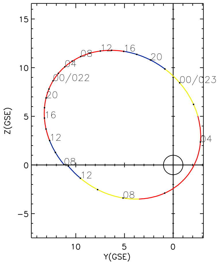
CLUSTER 2 orbit 2023 021 (01/21) 07:56 UT to 2023 023 (01/23) 14:06 UT
