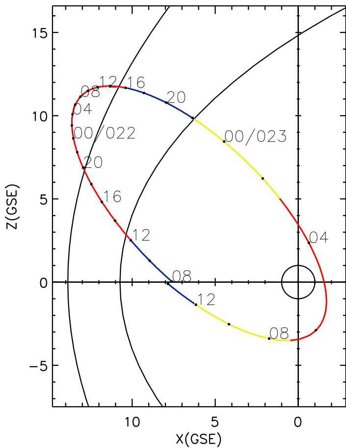
CLUSTER 2 orbit 2023 021 (01/21) 07:56 UT to 2023 023 (01/23) 14:06 UT
