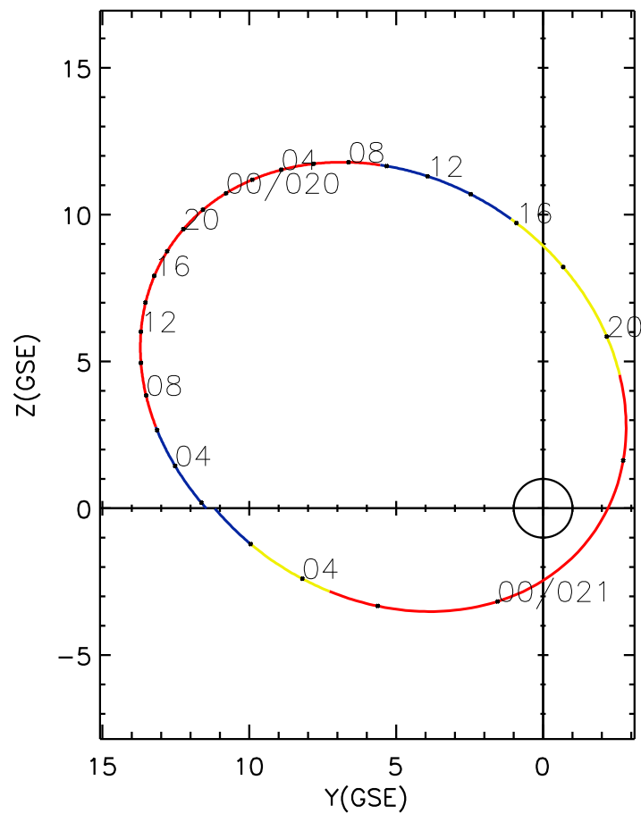
CLUSTER 2 orbit 2023 019 (01/19) 01:41 UT to 2023 021 (01/21) 07:56 UT
