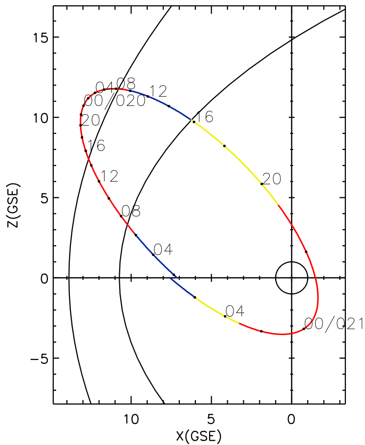
CLUSTER 2 orbit 2023 019 (01/19) 01:41 UT to 2023 021 (01/21) 07:56 UT
