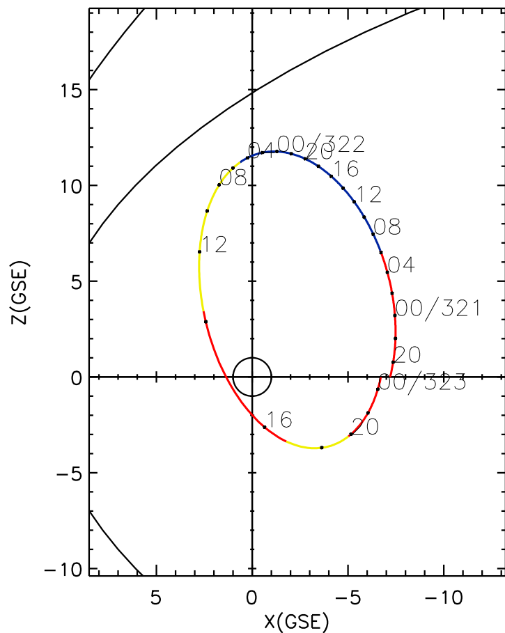
CLUSTER 2 orbit 2022 320 (11/16) 18:46 UT to 2022 323 (11/19) 01:01 UT
