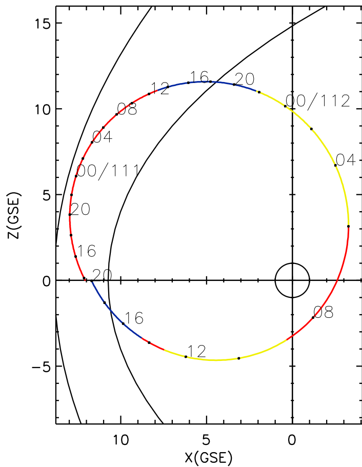
CLUSTER 2 orbit 2022 110 (04/20) 13:46 UT to 2022 112 (04/22) 20:01 UT
