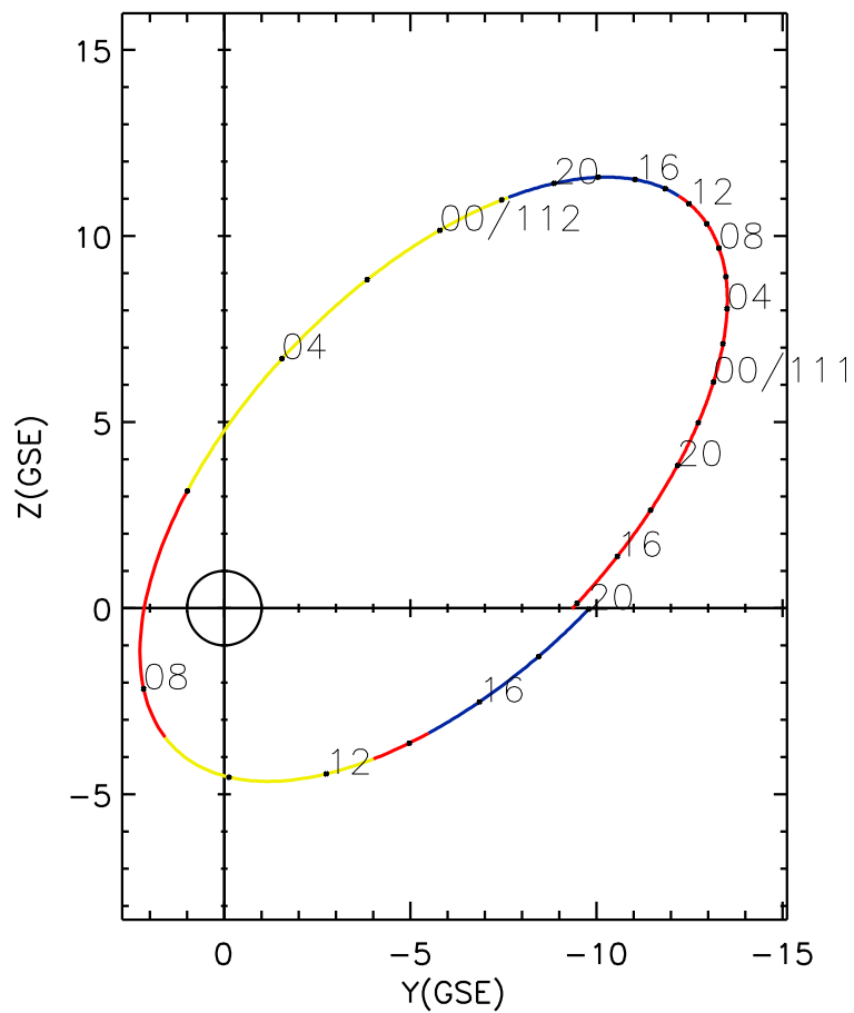
CLUSTER 2 orbit 2022 110 (04/20) 13:46 UT to 2022 112 (04/22) 20:01 UT
