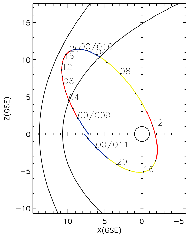
CLUSTER 2 orbit 2022 008 (01/08) 20:31 UT to 2022 011 (01/11) 02:51 UT
