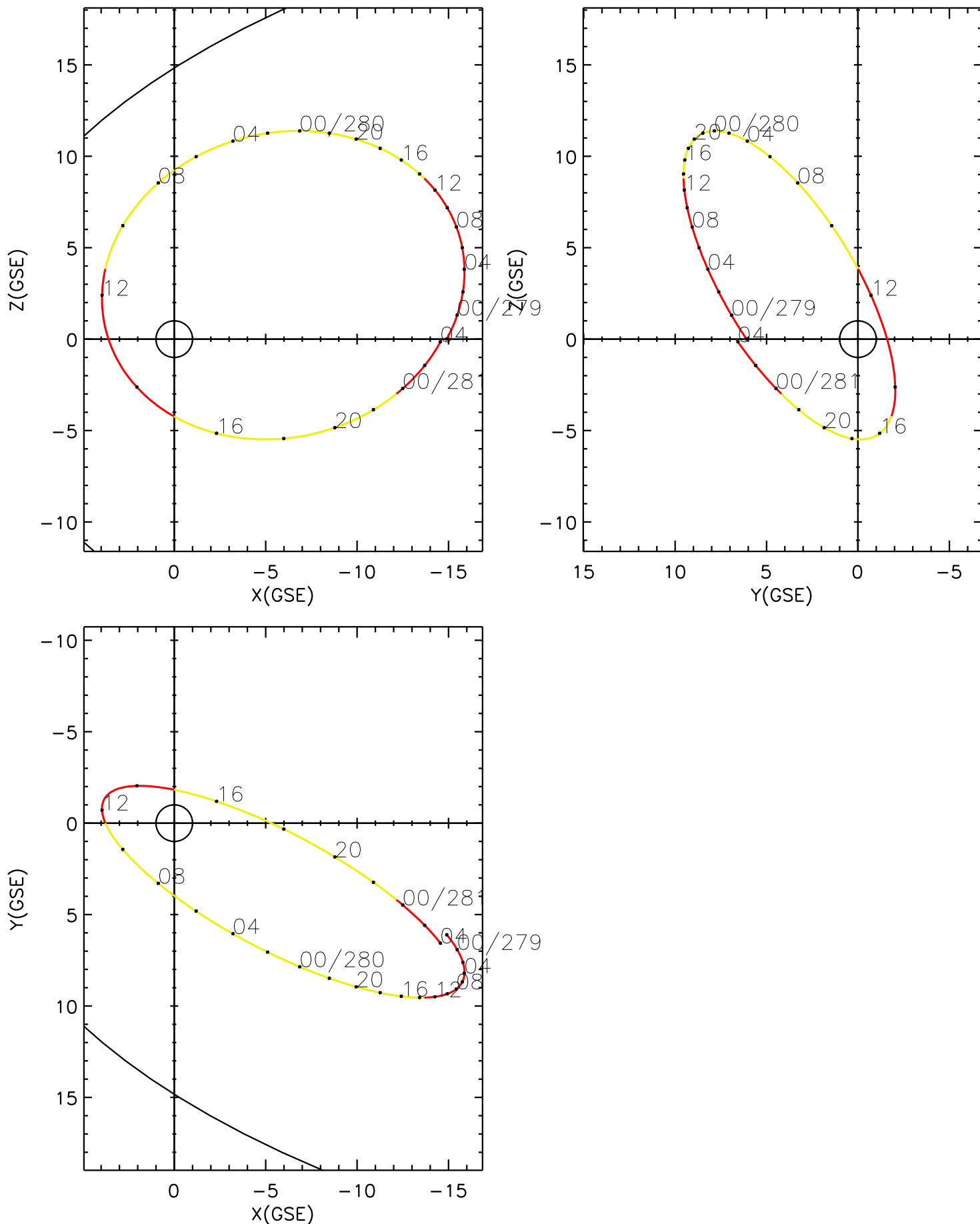
CLUSTER 2 orbit 2021 278 (10/05) 21:56 UT to 2021 281 (10/08) 04:11 UT
