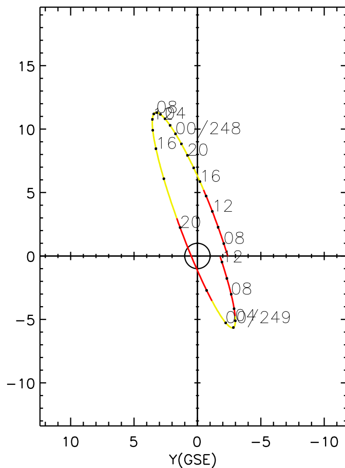
CLUSTER 2 orbit 2021 247 (09/04) 06:26 UT to 2021 249 (09/06) 12:41 UT
