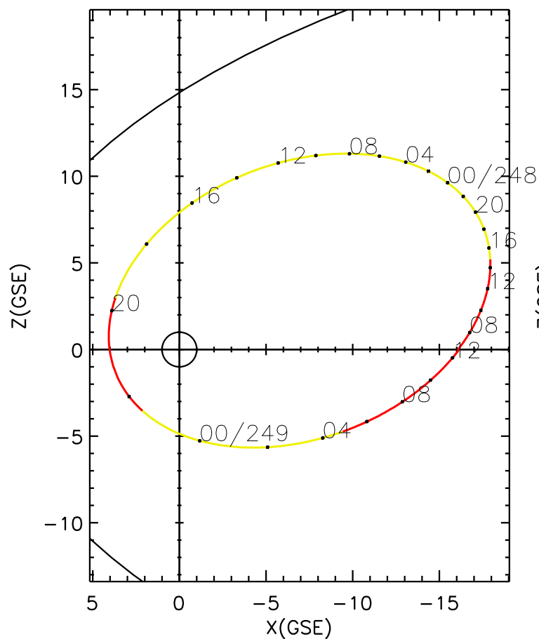
CLUSTER 2 orbit 2021 247 (09/04) 06:26 UT to 2021 249 (09/06) 12:41 UT
