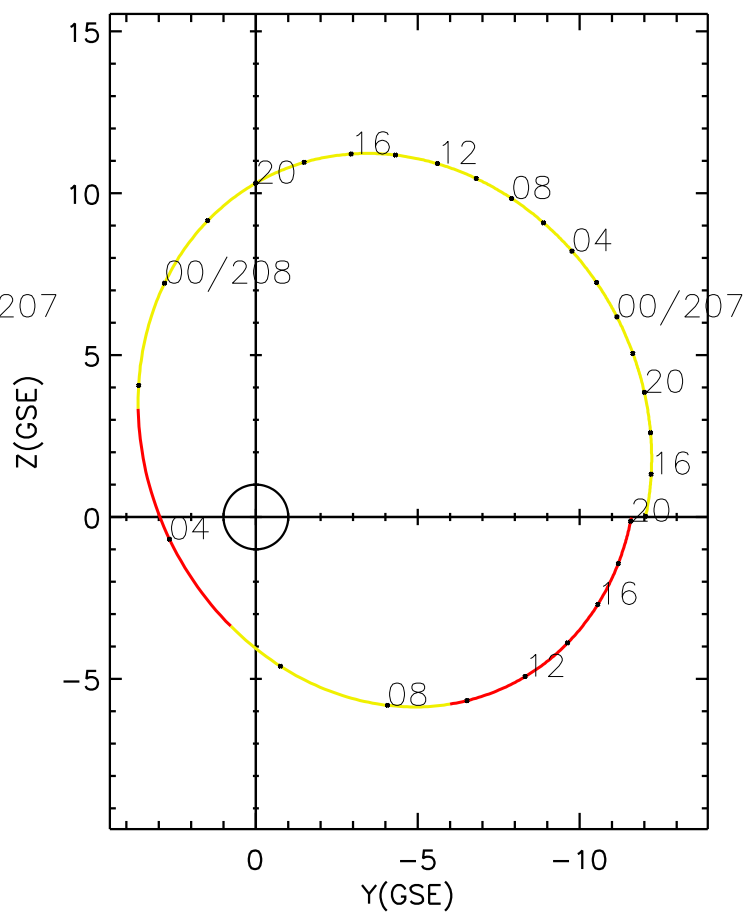
CLUSTER 2 orbit 2021 206 (07/25) 13:56 UT to 2021 208 (07/27) 20:11 UT
