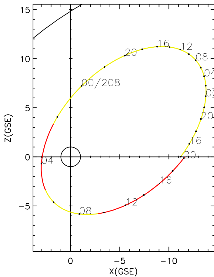
CLUSTER 2 orbit 2021 206 (07/25) 13:56 UT to 2021 208 (07/27) 20:11 UT
