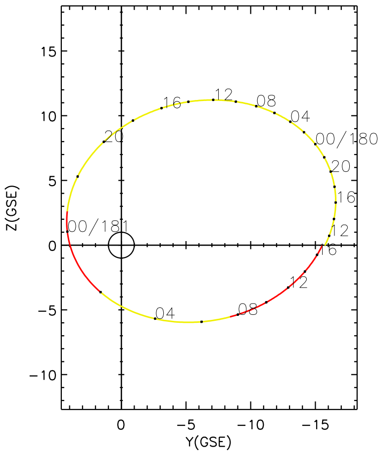
CLUSTER 2 orbit 2021 179 (06/28) 10:51 UT to 2021 181 (06/30) 17:06 UT
