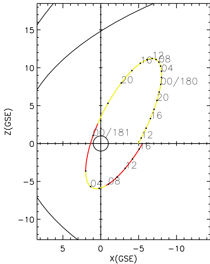
CLUSTER 2 orbit 2021 179 (06/28) 10:51 UT to 2021 181 (06/30) 17:06 UT
