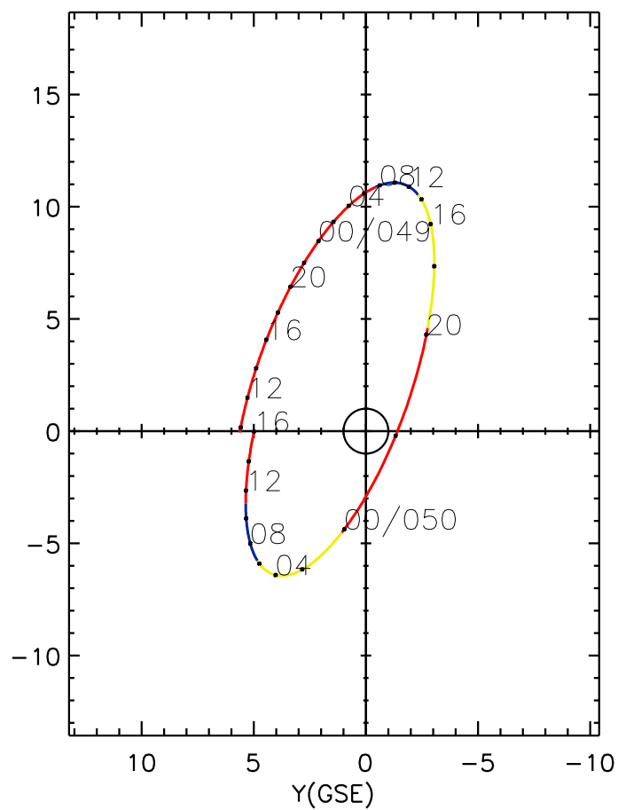
CLUSTER 2 orbit 2021 048 (02/17) 09:41 UT to 2021 050 (02/19) 16:01 UT
