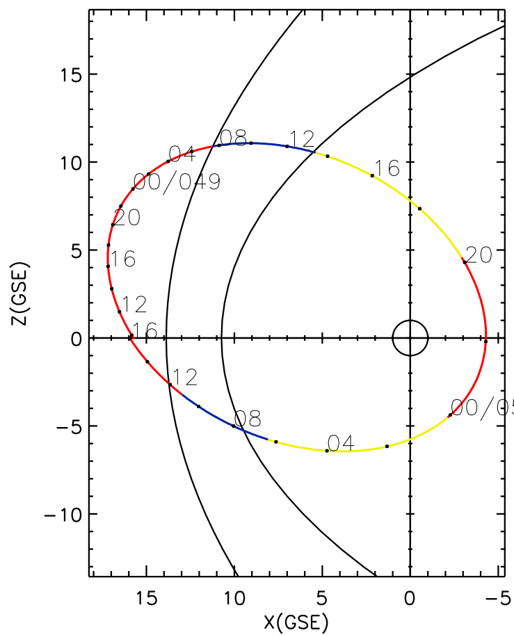
CLUSTER 2 orbit 2021 048 (02/17) 09:41 UT to 2021 050 (02/19) 16:01 UT
