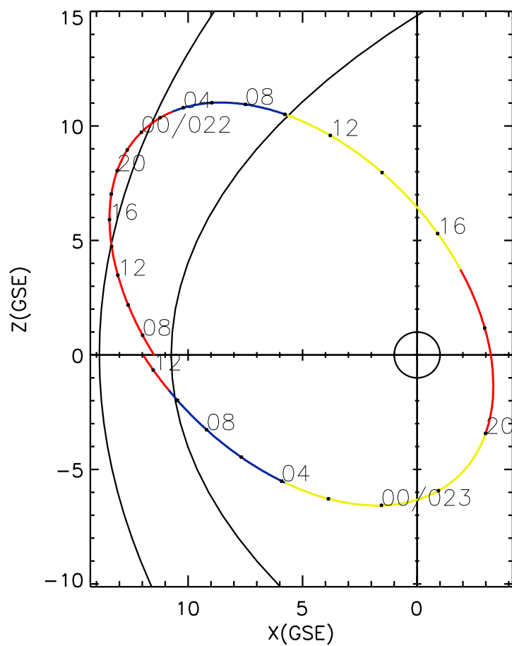
CLUSTER 2 orbit 2021 021 (01/21) 06:41 UT to 2021 023 (01/23) 12:56 UT
