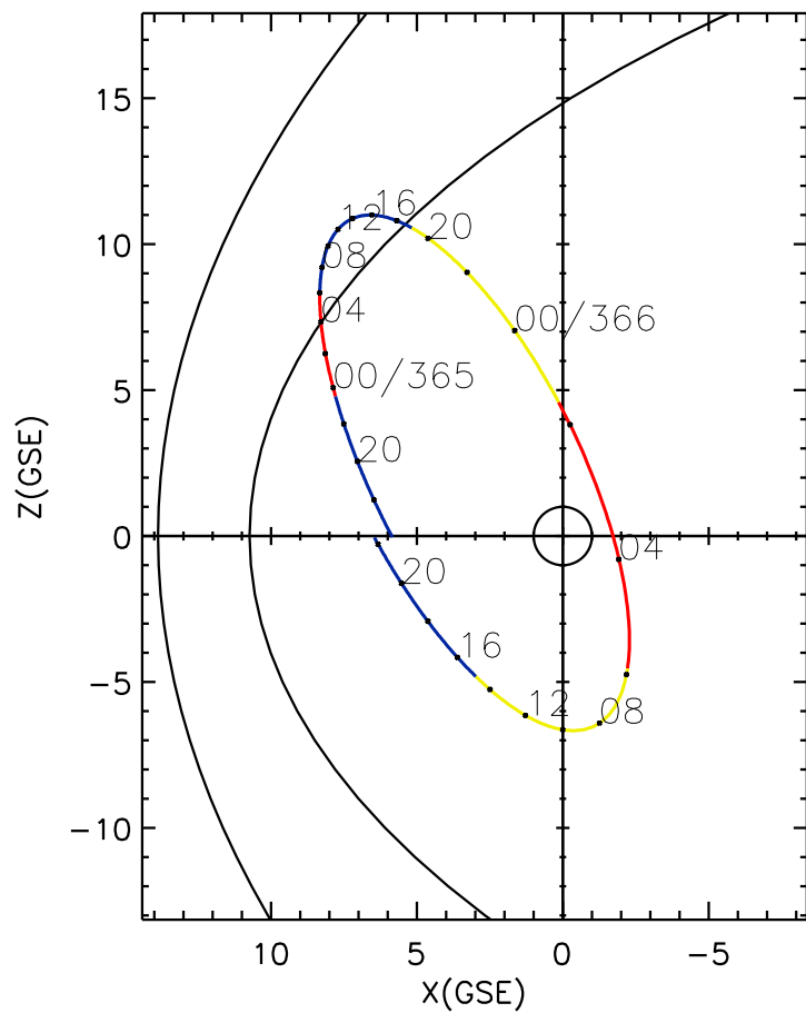
CLUSTER 2 orbit 2020 364 (12/29) 16:06 UT to 2020 366 (12/31) 22:21 UT
