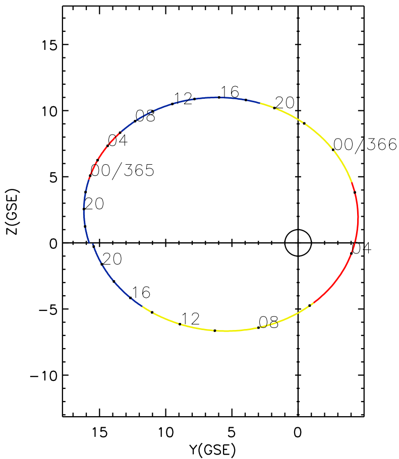
CLUSTER 2 orbit 2020 364 (12/29) 16:06 UT to 2020 366 (12/31) 22:21 UT
