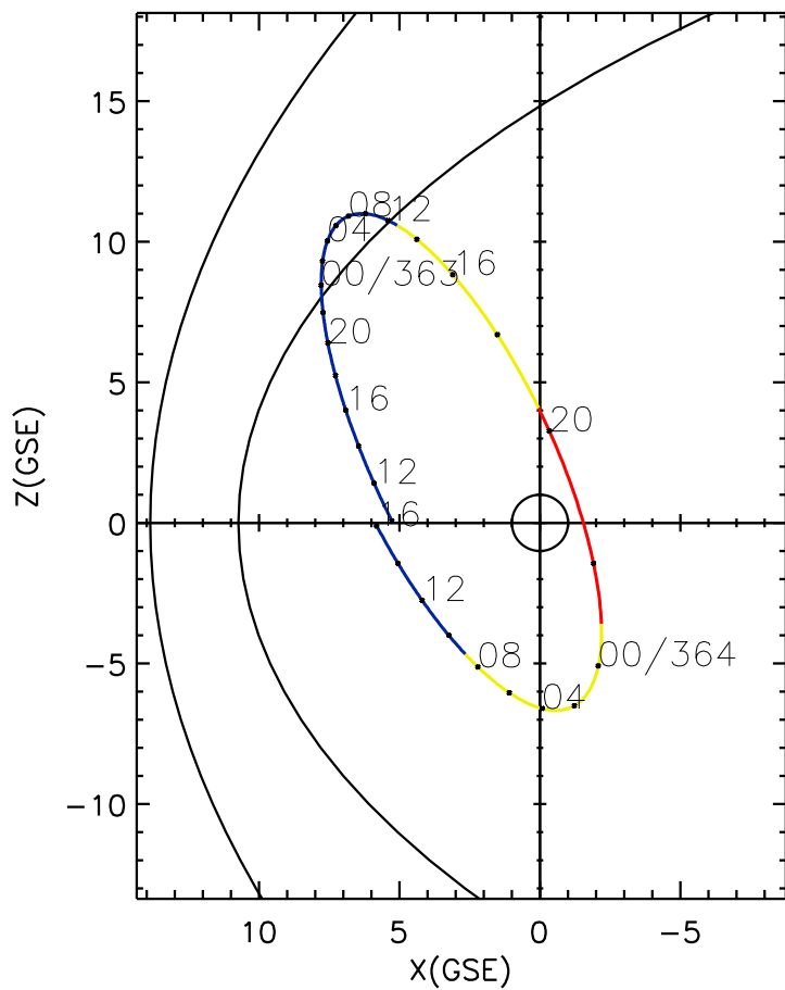
CLUSTER 2 orbit 2020 362 (12/27) 09:51 UT to 2020 364 (12/29) 16:06 UT
