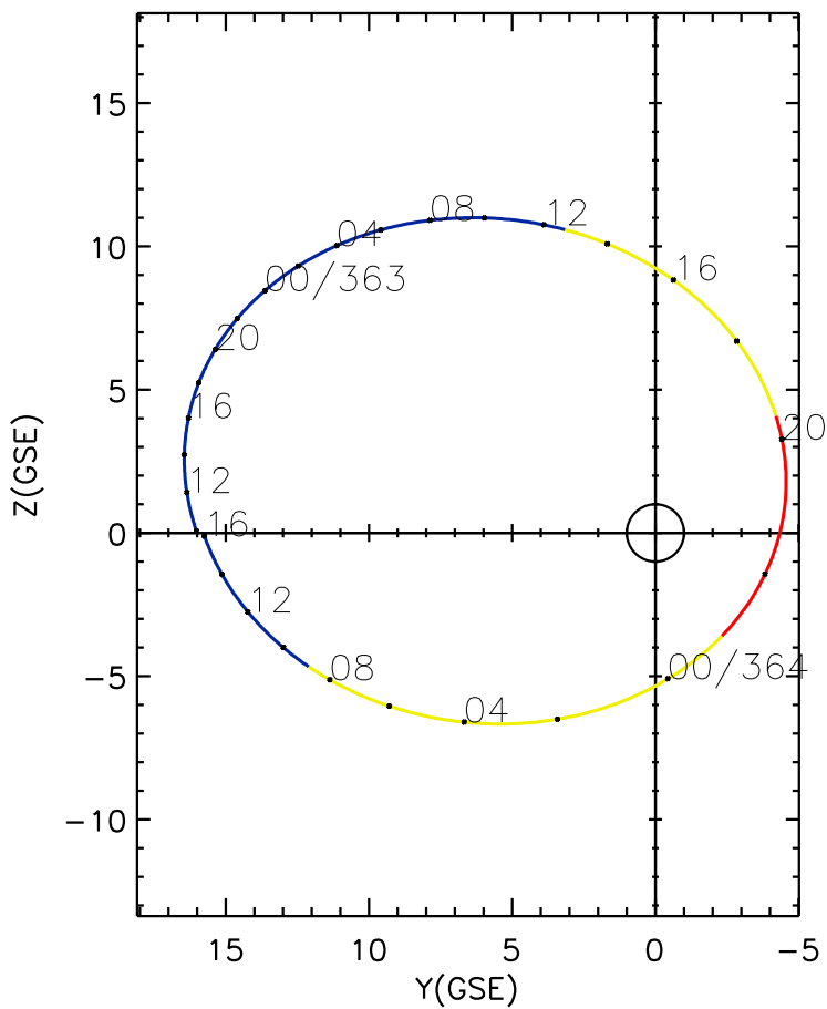
CLUSTER 2 orbit 2020 362 (12/27) 09:51 UT to 2020 364 (12/29) 16:06 UT
