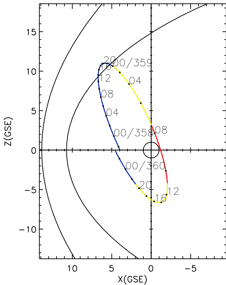
CLUSTER 2 orbit 2020 357 (12/22) 21:21 UT to 2020 360 (12/25) 03:36 UT
