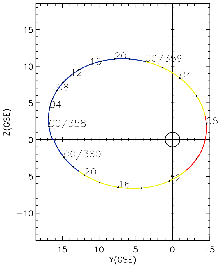
CLUSTER 2 orbit 2020 357 (12/22) 21:21 UT to 2020 360 (12/25) 03:36 UT
