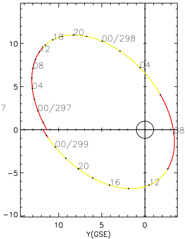
CLUSTER 2 orbit 2020 296 (10/22) 20:41 UT to 2020 299 (10/25) 02:56 UT
