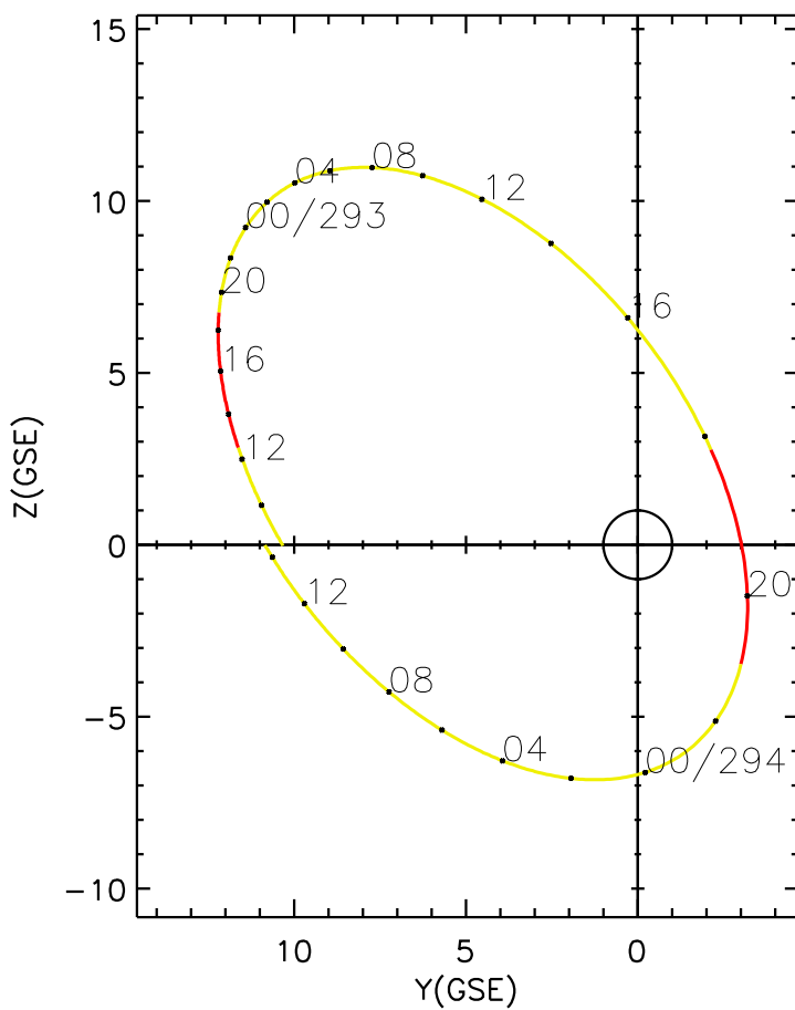
CLUSTER 2 orbit 2020 292 (10/18) 08:16 UT to 2020 294 (10/20) 14:31 UT
