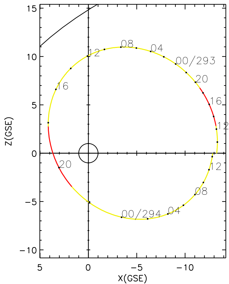
CLUSTER 2 orbit 2020 292 (10/18) 08:16 UT to 2020 294 (10/20) 14:31 UT
