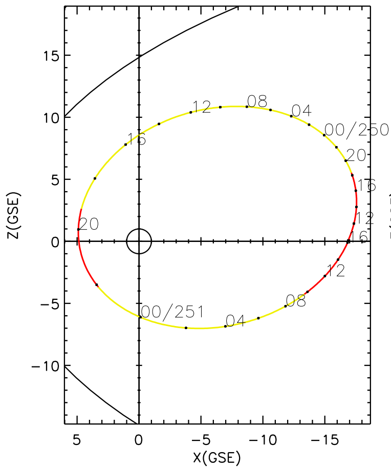
CLUSTER 2 orbit 2020 249 (09/05) 09:51 UT to 2020 251 (09/07) 16:06 UT
