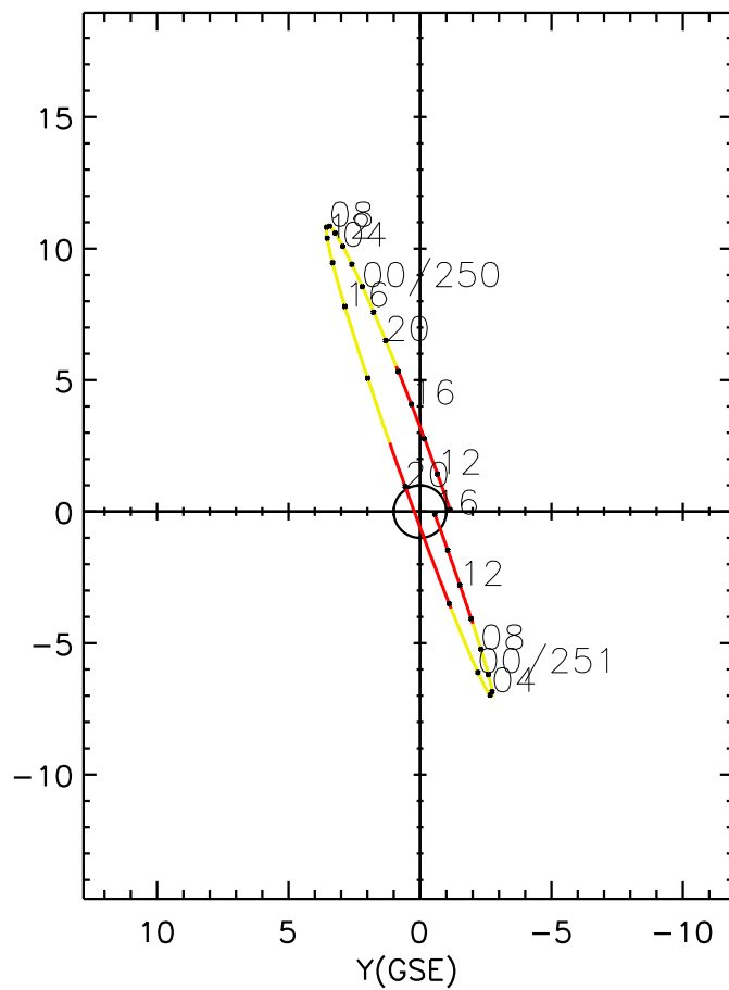
CLUSTER 2 orbit 2020 249 (09/05) 09:51 UT to 2020 251 (09/07) 16:06 UT
