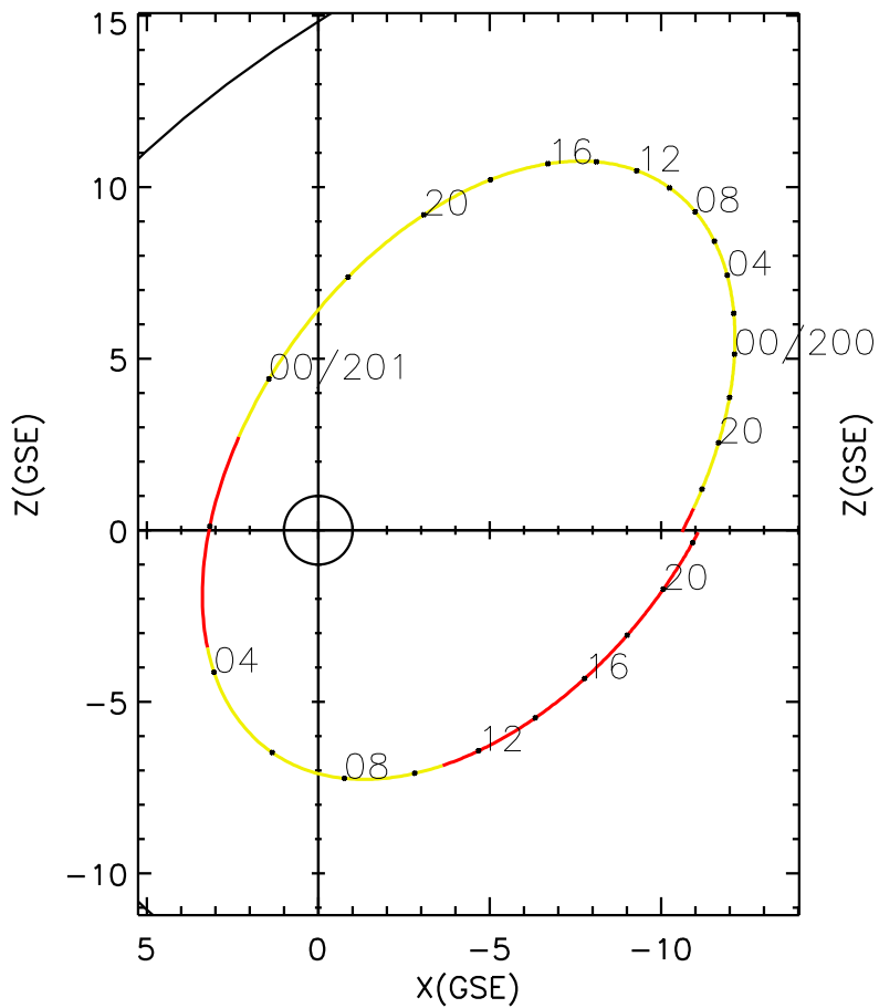
CLUSTER 2 orbit 2020 199 (07/17) 16:11 UT to 2020 201 (07/19) 22:26 UT
