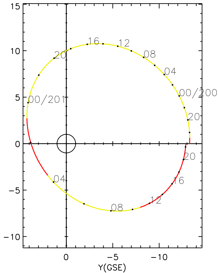
CLUSTER 2 orbit 2020 199 (07/17) 16:11 UT to 2020 201 (07/19) 22:26 UT
