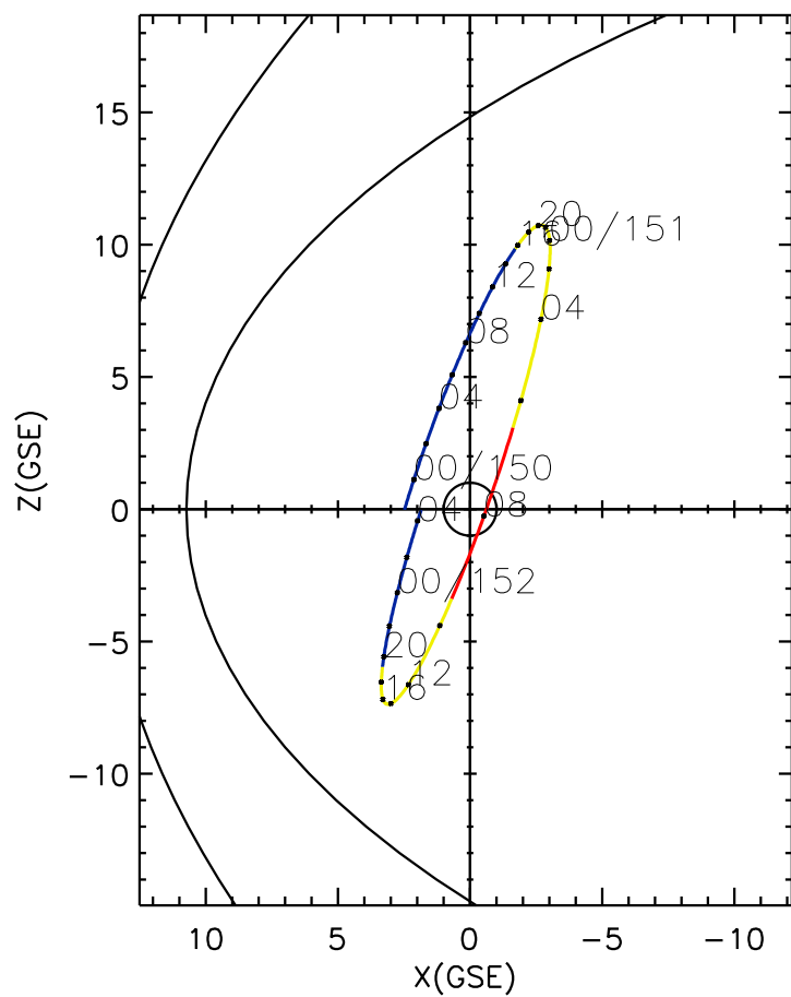
CLUSTER 2 orbit 2020 149 (05/28) 22:21 UT to 2020 152 (05/31) 04:36 UT
