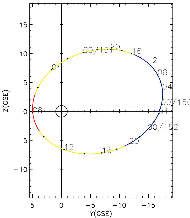
CLUSTER 2 orbit 2020 149 (05/28) 22:21 UT to 2020 152 (05/31) 04:36 UT
