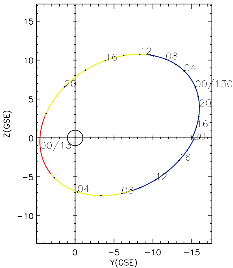
CLUSTER 2 orbit 2020 129 (05/08) 13:56 UT to 2020 131 (05/10) 20:11 UT
