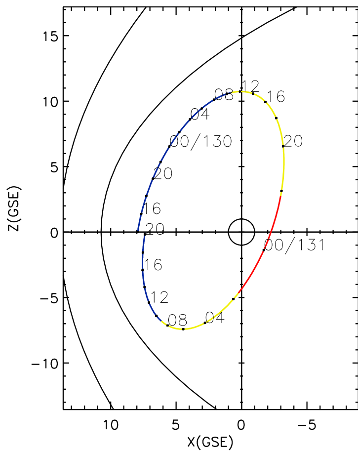
CLUSTER 2 orbit 2020 129 (05/08) 13:56 UT to 2020 131 (05/10) 20:11 UT
