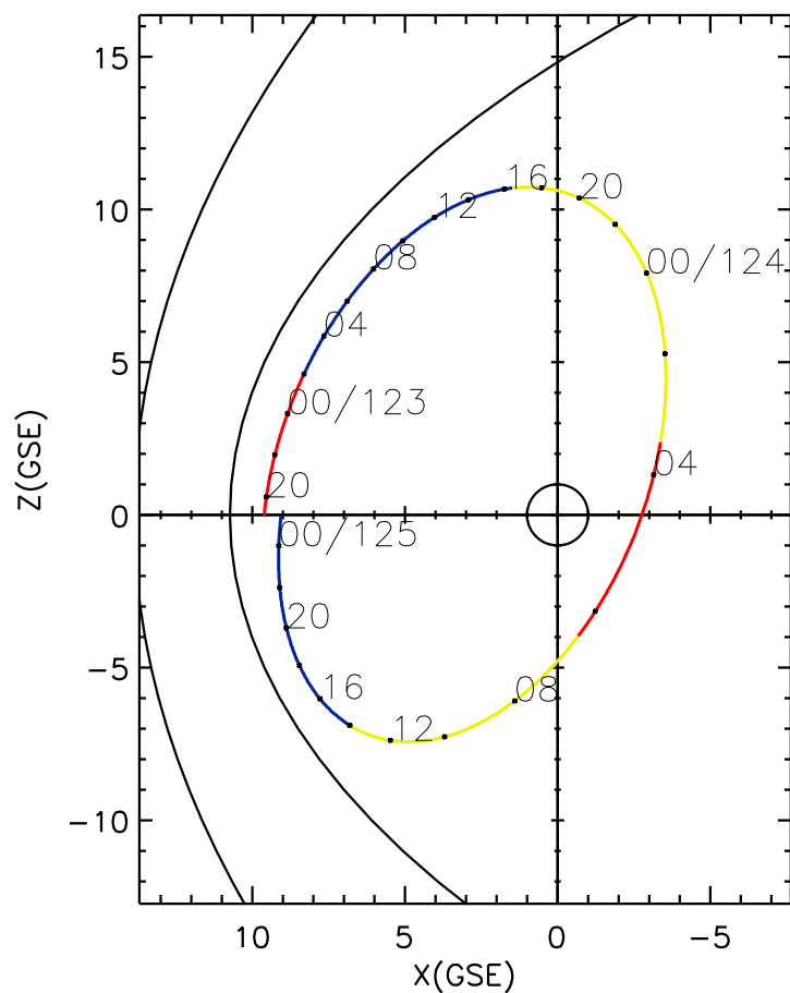
CLUSTER 2 orbit 2020 122 (05/01) 19:06 UT to 2020 125 (05/04) 01:26 UT
