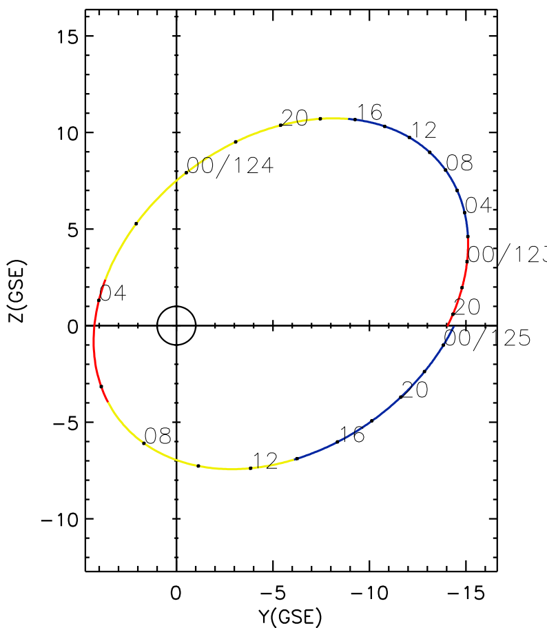
CLUSTER 2 orbit 2020 122 (05/01) 19:06 UT to 2020 125 (05/04) 01:26 UT
