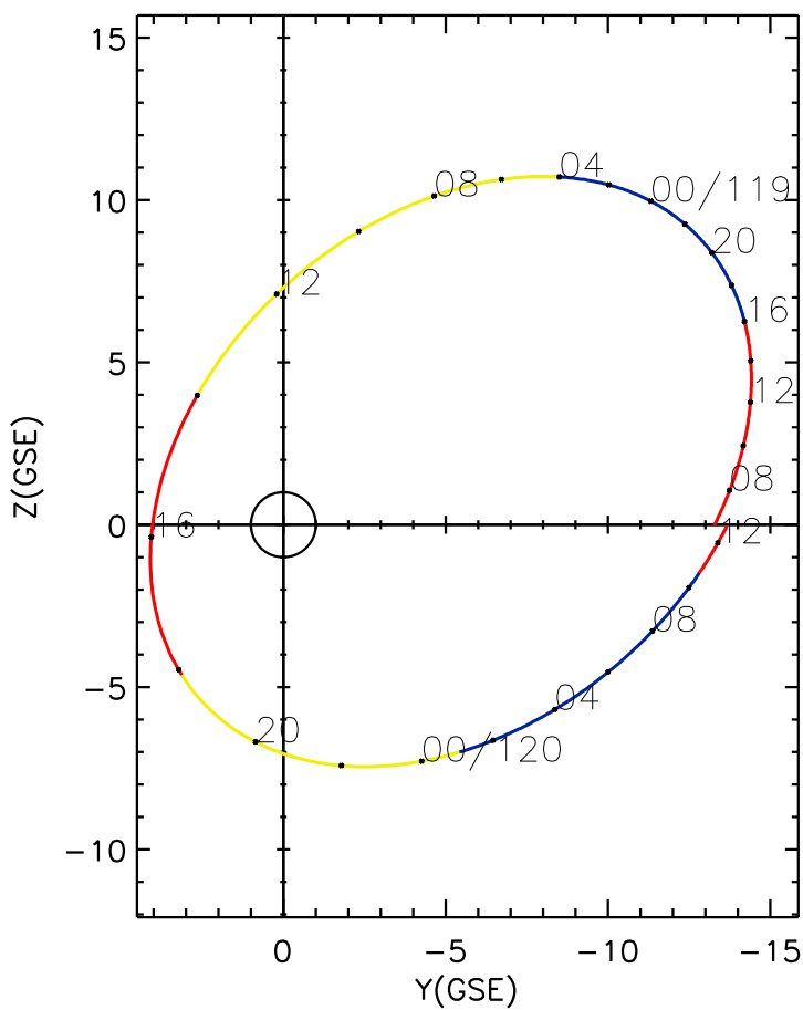
CLUSTER 2 orbit 2020 118 (04/27) 06:26 UT to 2020 120 (04/29) 12:46 UT
