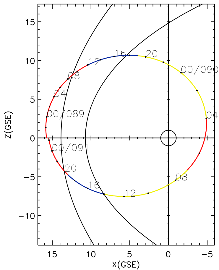
CLUSTER 2 orbit 2020 088 (03/28) 20:01 UT to 2020 091 (03/31) 02:21 UT
