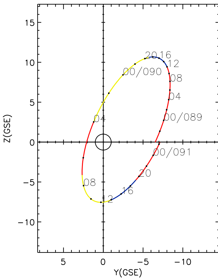
CLUSTER 2 orbit 2020 088 (03/28) 20:01 UT to 2020 091 (03/31) 02:21 UT
